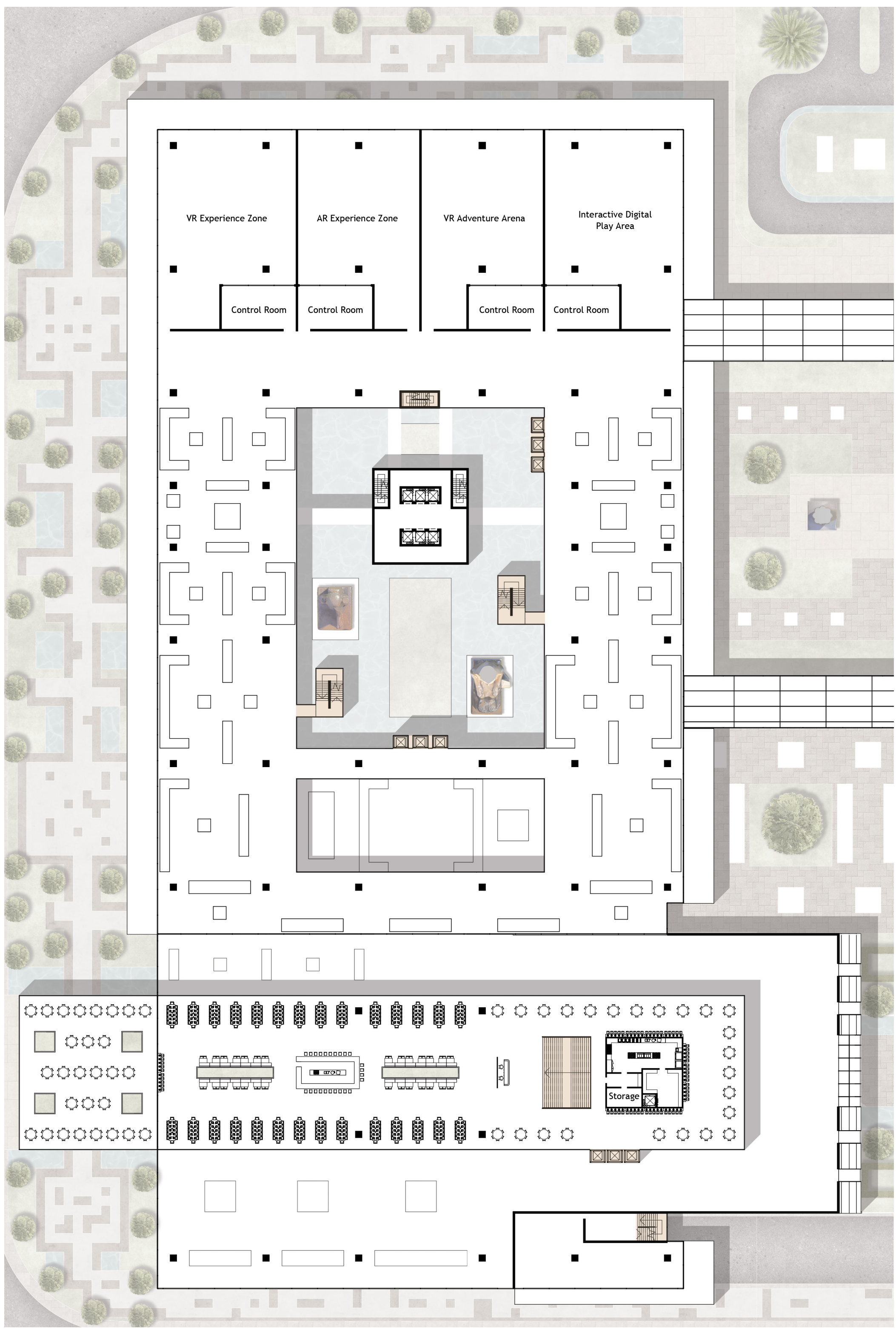
FIRST FLOOR PLAN 1:500
