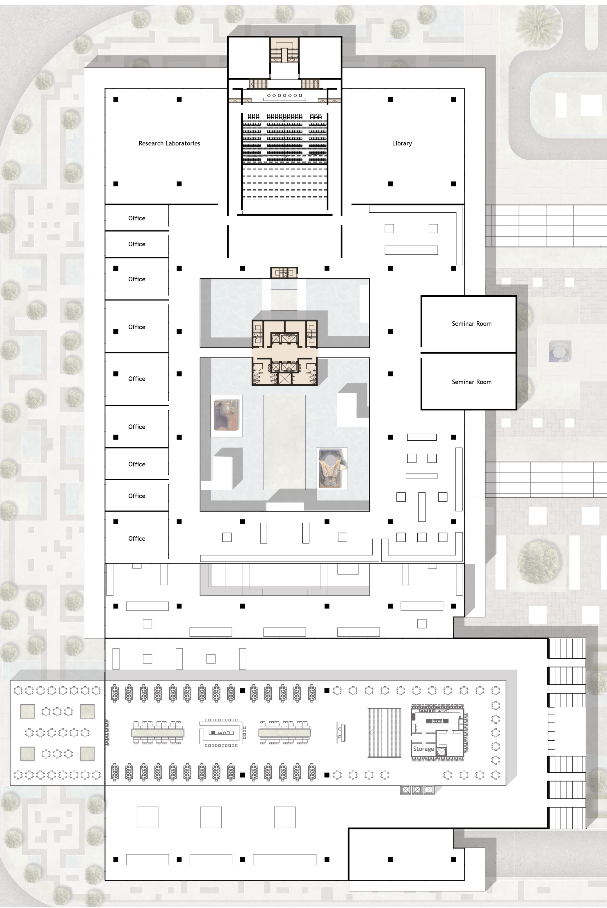
THIRD FLOOR PLAN 1:500
