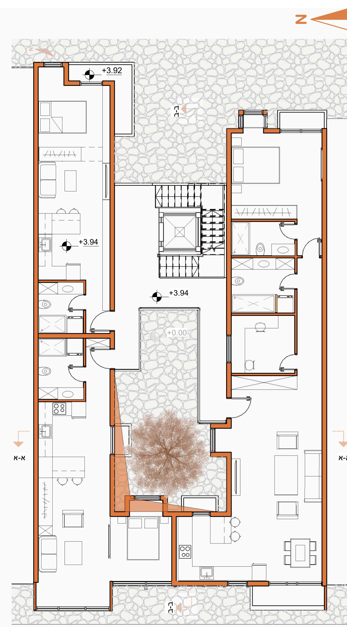
First Floor Plan 1:100
