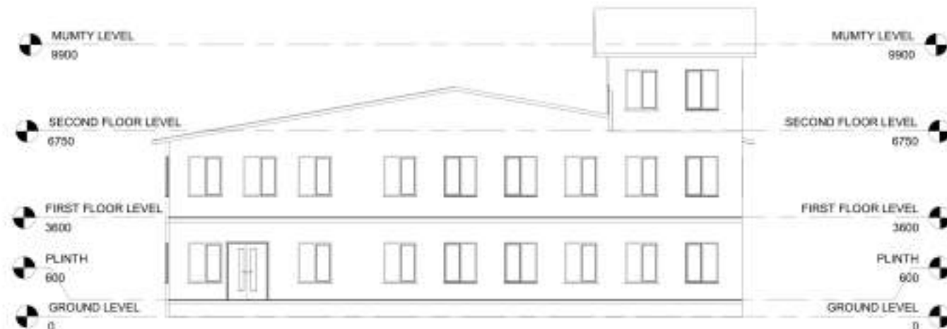
WEST ELEVATION
