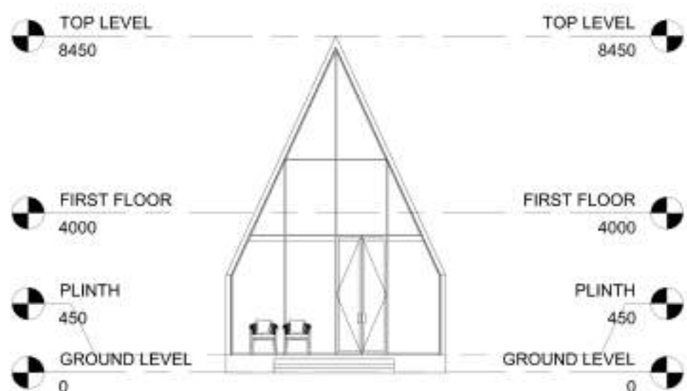
SOUTH ELEVATION
