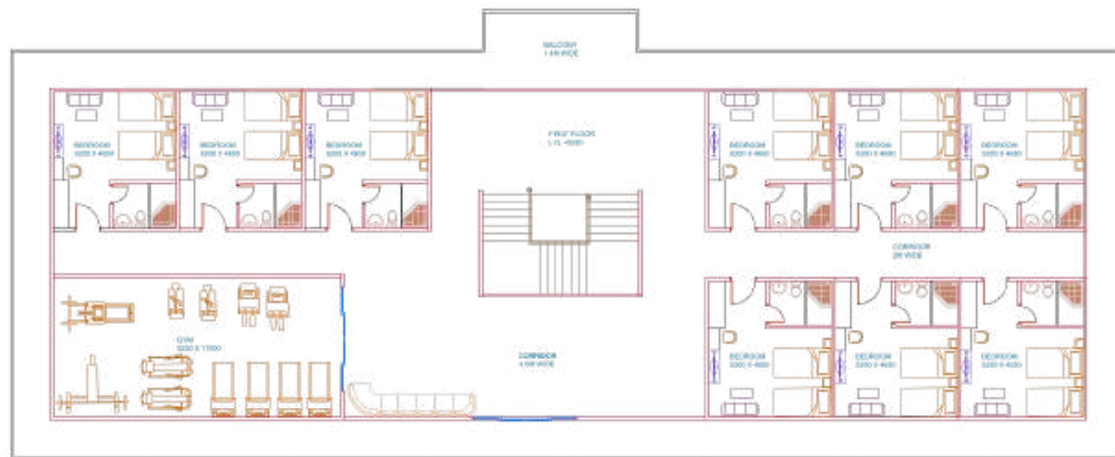
FIRST FLOOR
