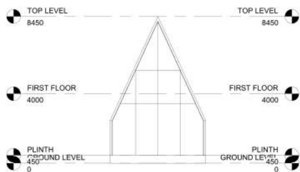
NORTH ELEVATION
