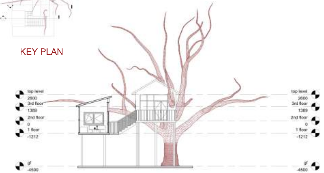
SECTION AA
