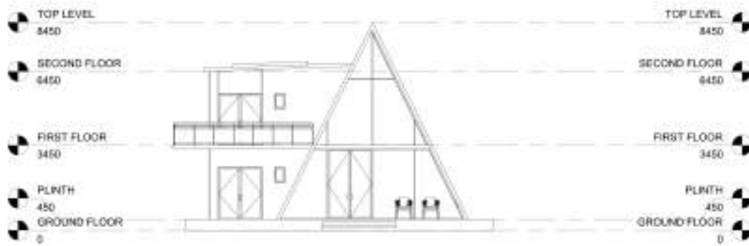
SOUTH ELEVATION
