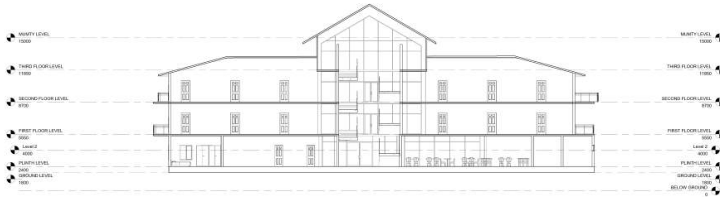
SECTION CC
