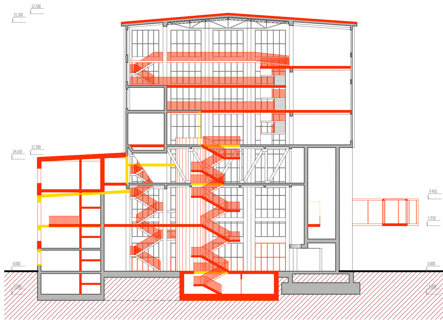
REZ AA
