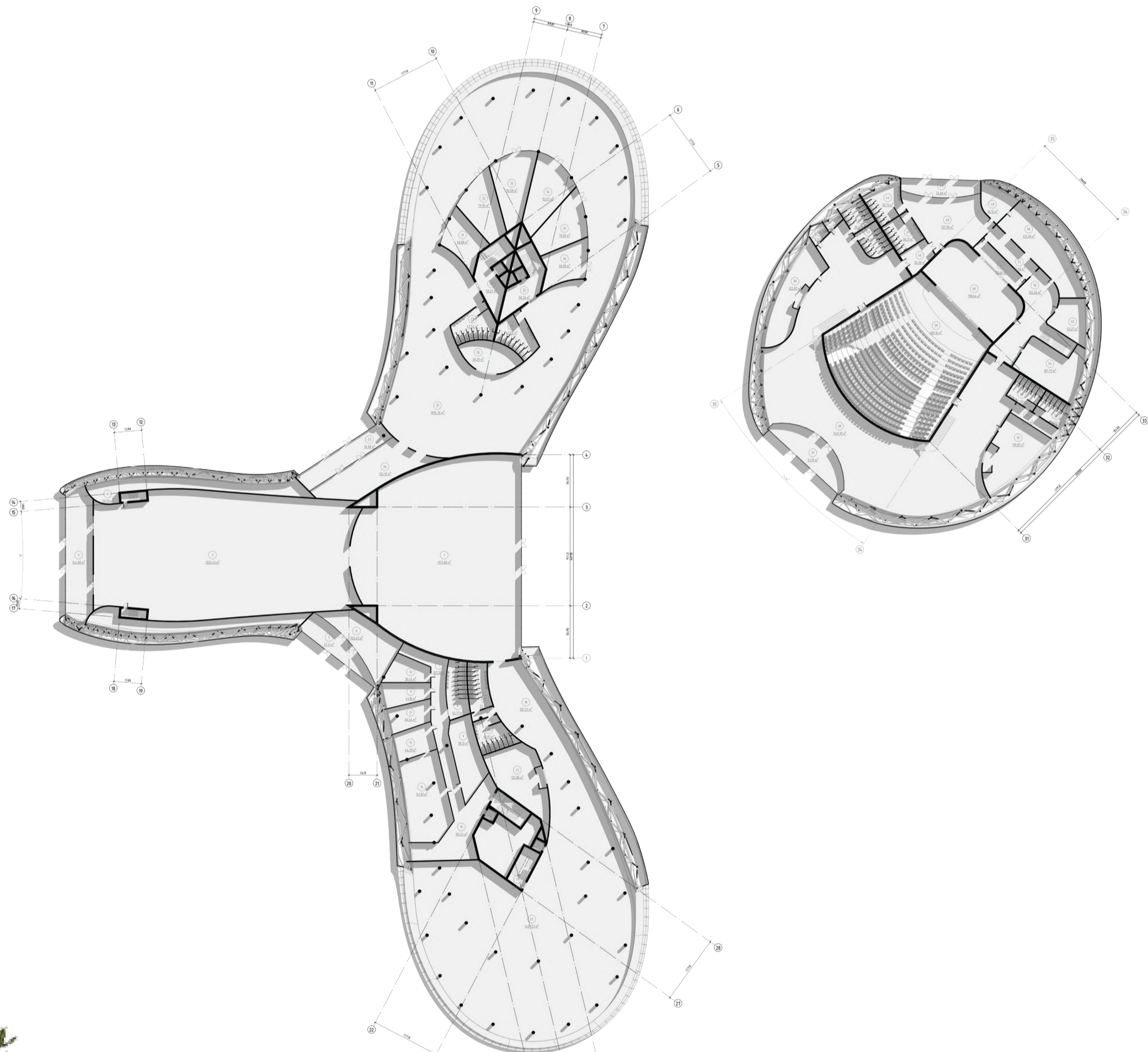
First floor
