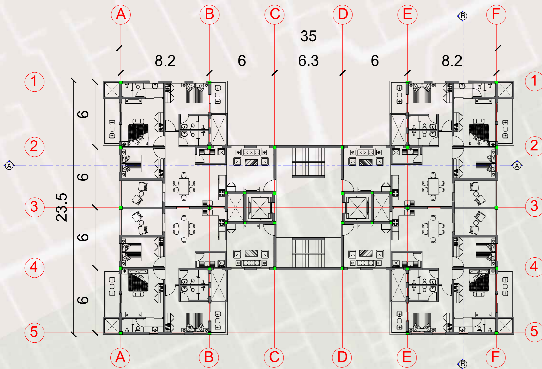
BLOCK FLOOR PLAN
