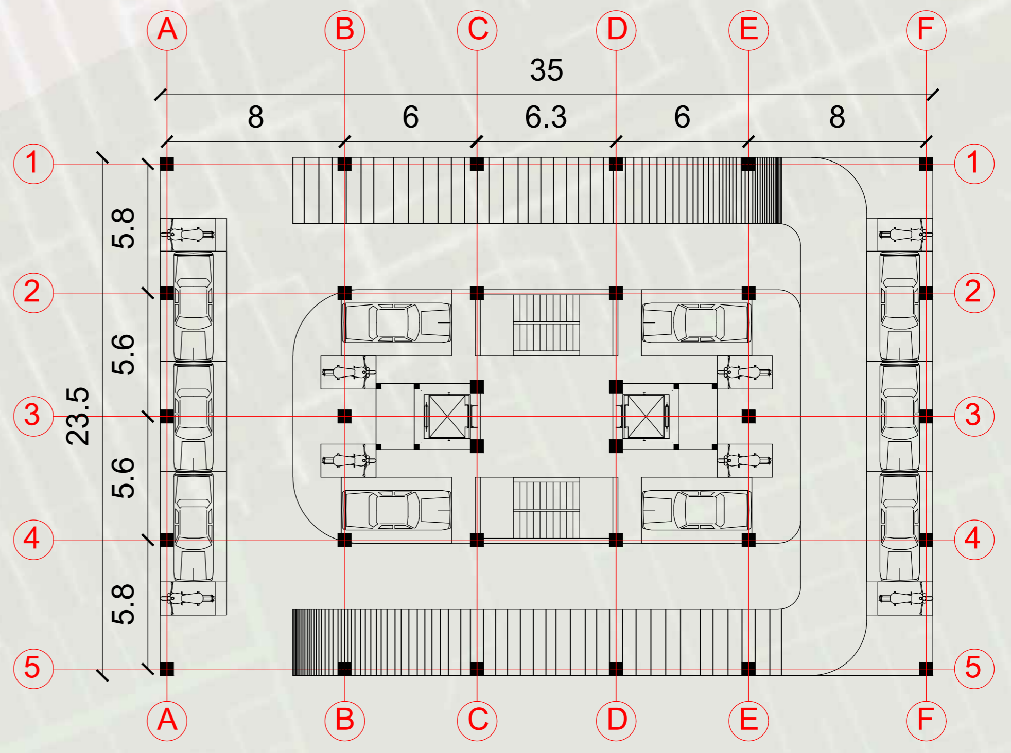
TYPICAL STILT FLOOR PLAN
