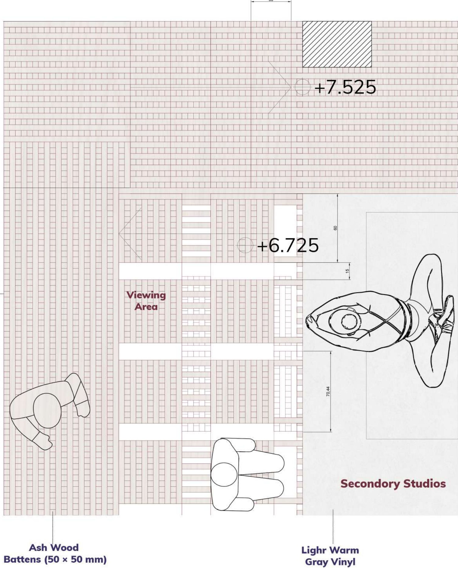
1/20 +7.525 Plan
