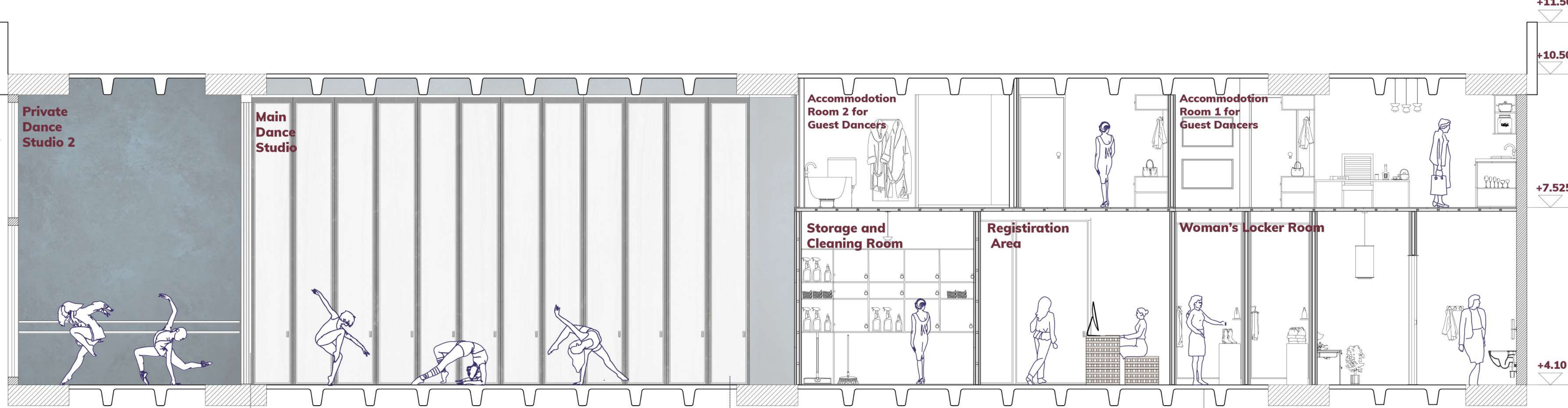
1/50 Aa Section
