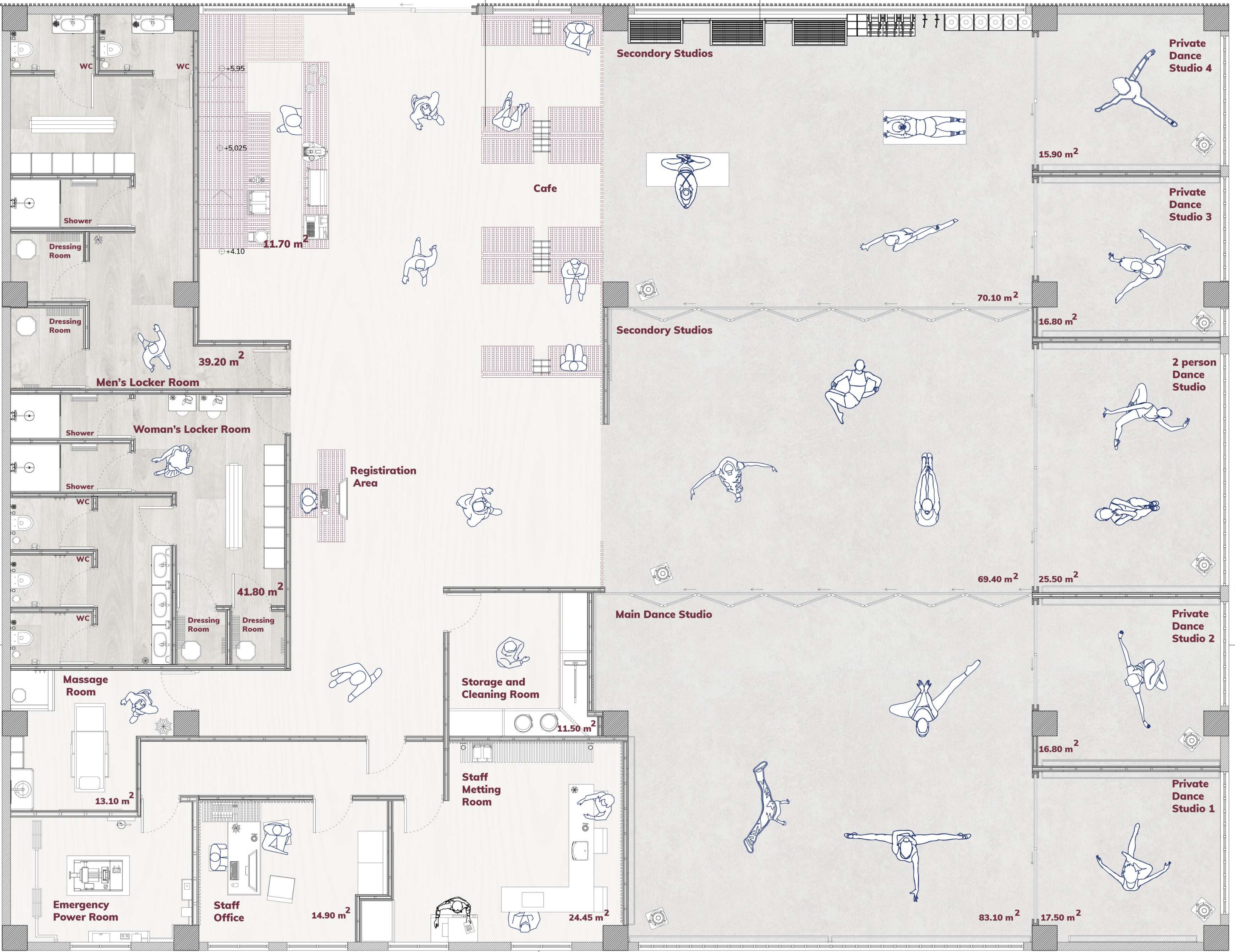
1/50 +5.95 Plan
