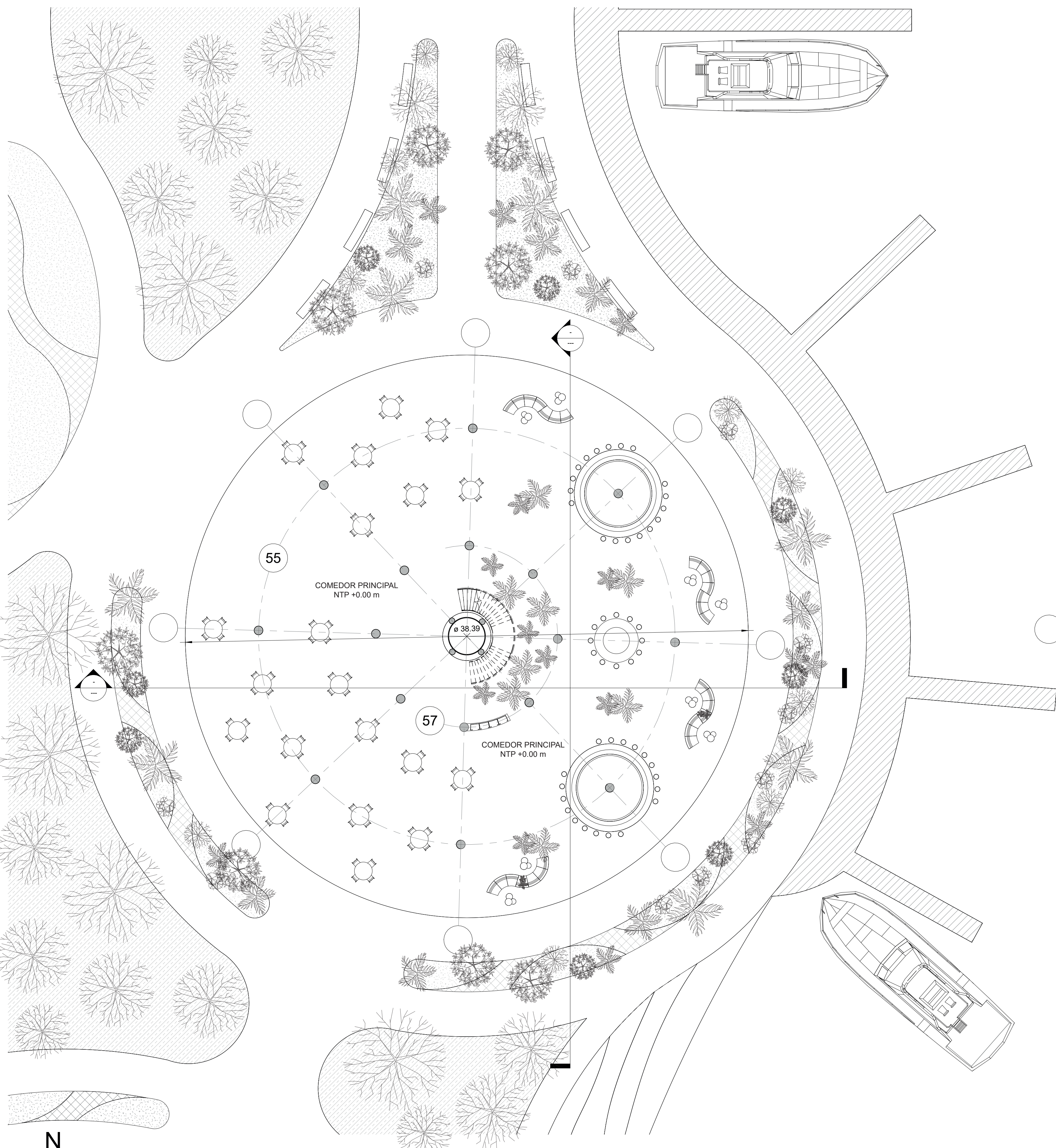
1 RESTAURANT LEVEL 1 +0.00 m SCALE 1 : 150
