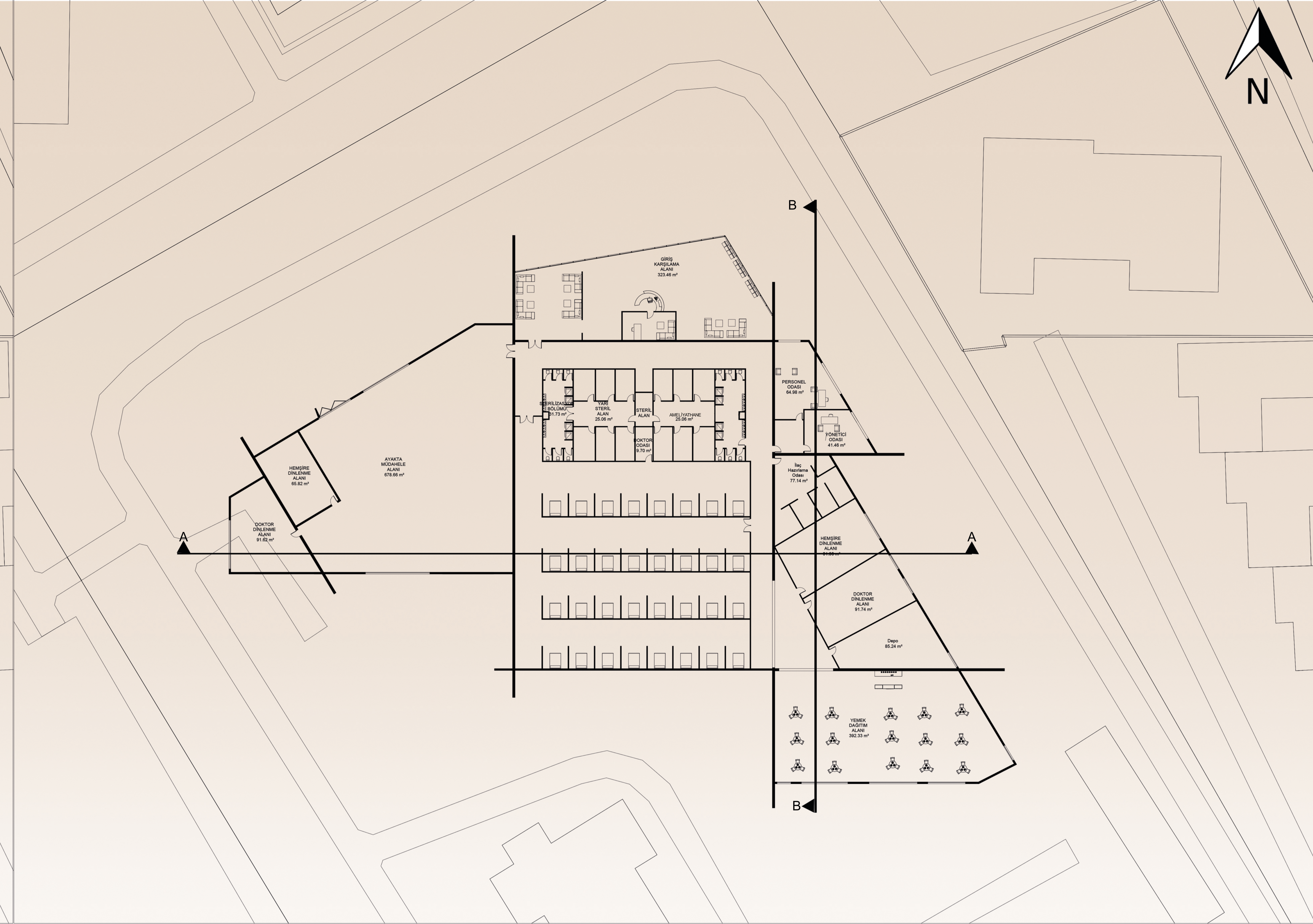
FIELD HOSPITAL PLAN 1:200
