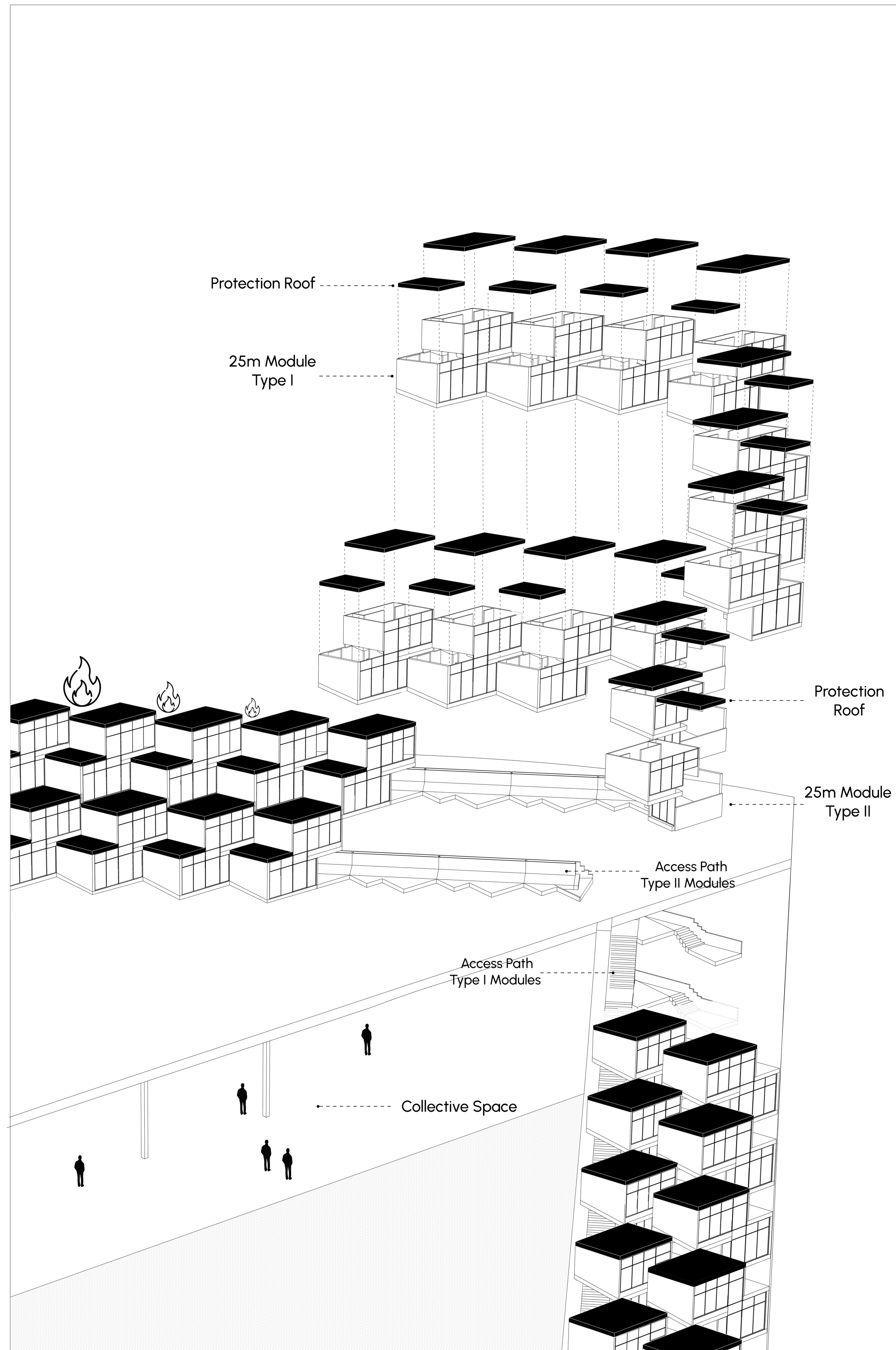
The exploded composition reveals a vertical stratification of defensive and functional layers. Protective walls and fire-resistant roofs define a spatial system where security, modularity, and habitability are tightly interwoven.
