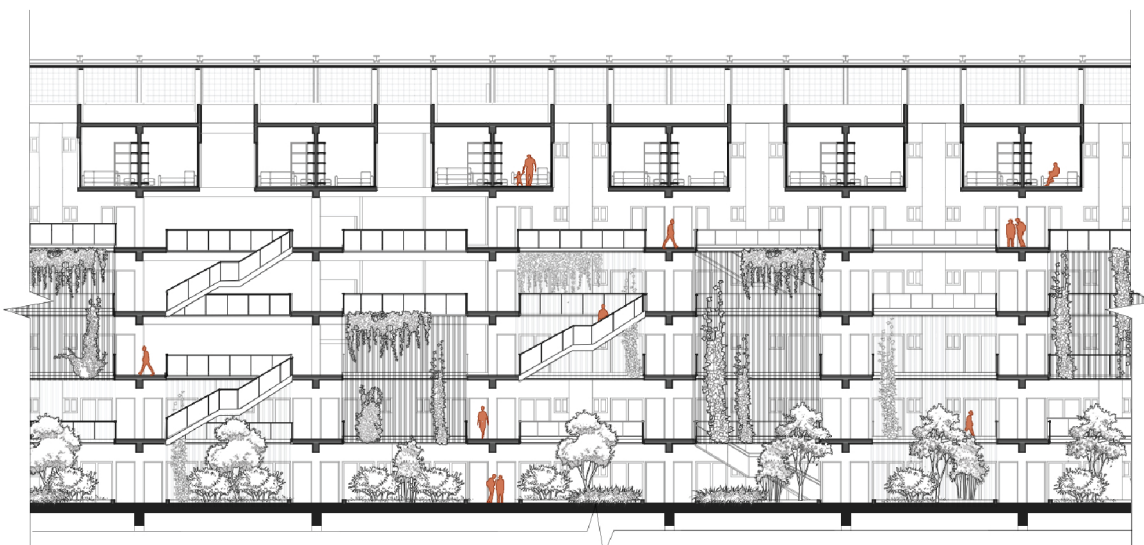
SECTION BB 0 2 4 10m
