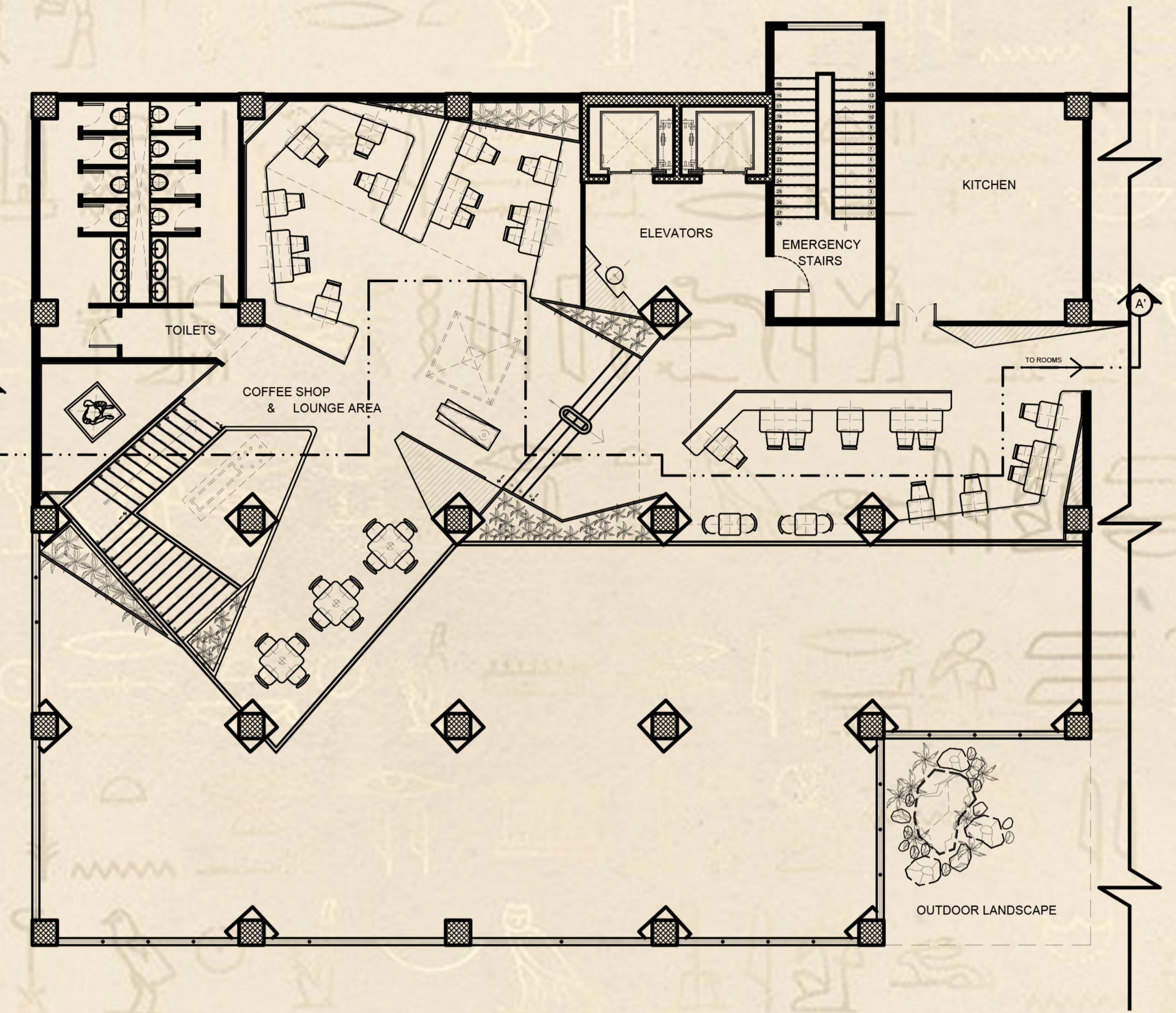
PLAN MEZZANINE FLOOR (1:100)
