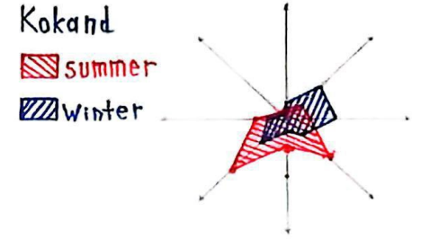
Wind rose
