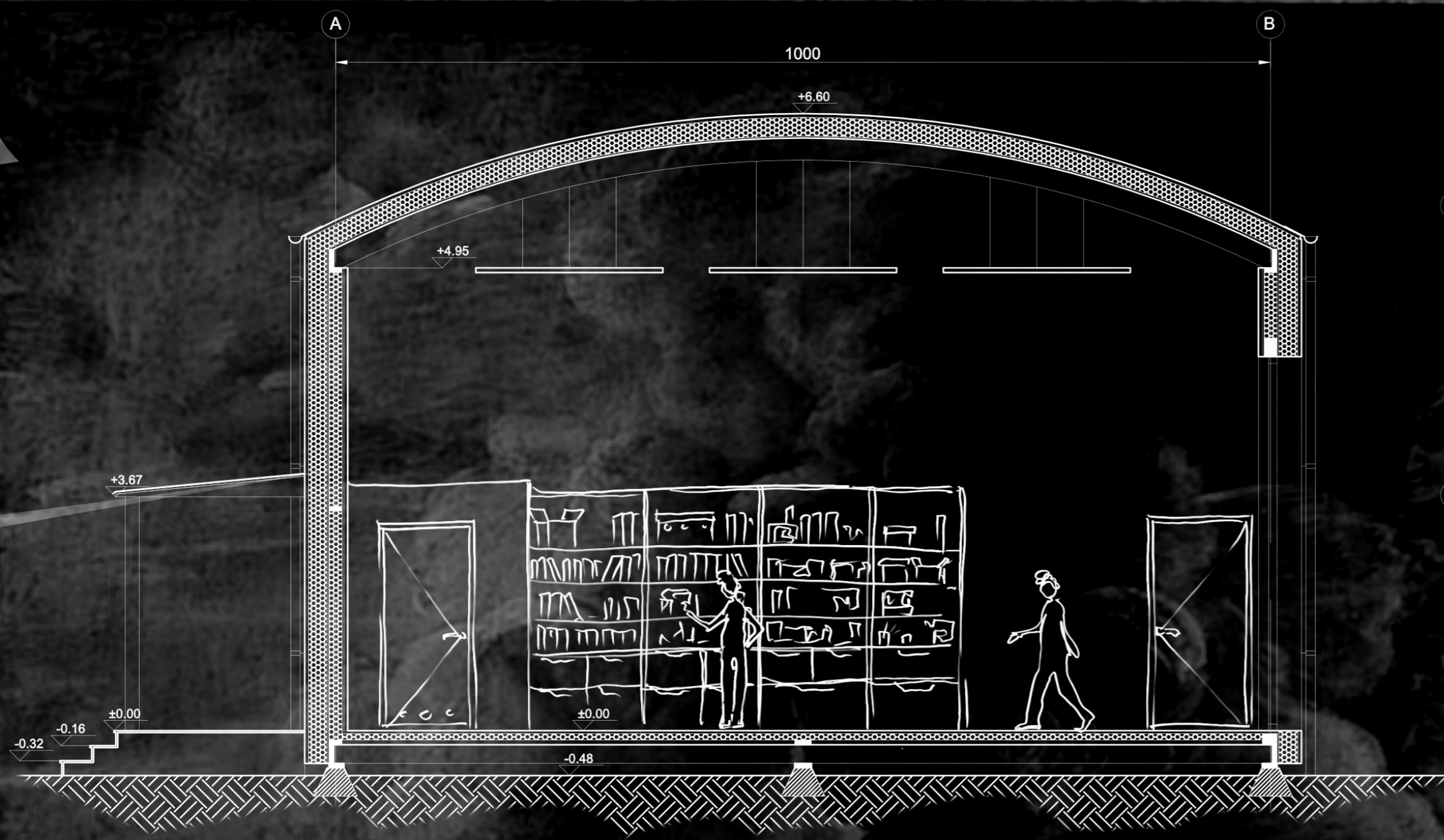
SECTION E-E 1:50
