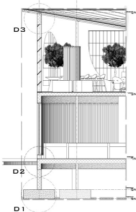
TYPICAL SECTION SCALE 1:10
