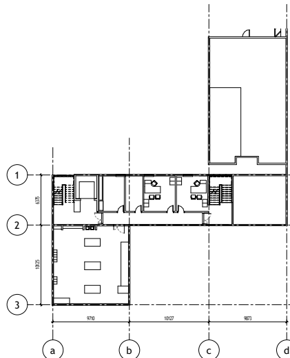
2 First Floor 1 : 200
