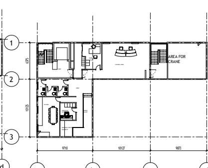
6 Fifth Floor 1 : 200
