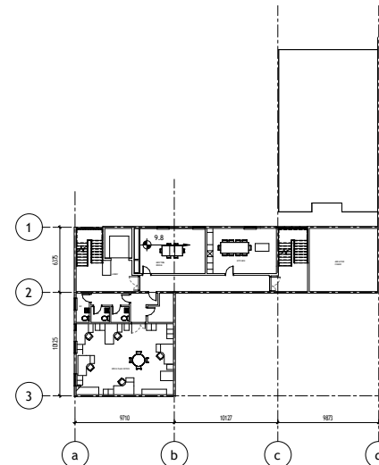
3 Second Floor 1 : 200
