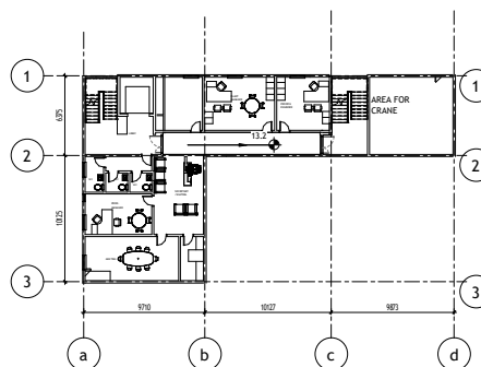
4 Third Floor 1 : 200
