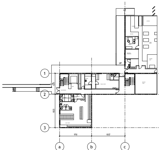
1 Ground Floor 1 : 200
