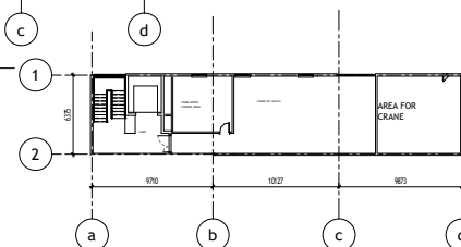
7 Sixth Floor 1 : 200
