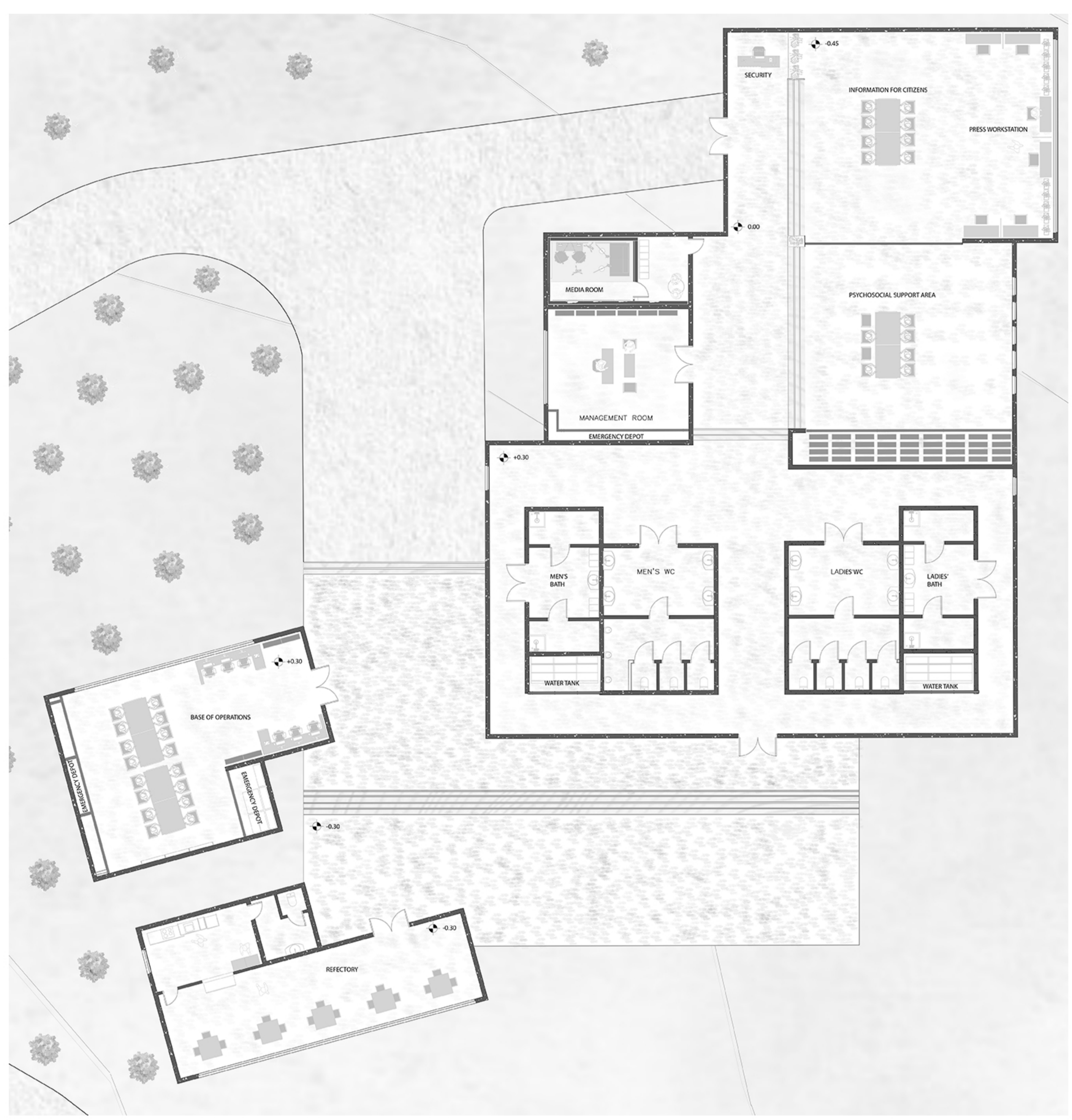
TRANSFORMED PLAN 1/100
