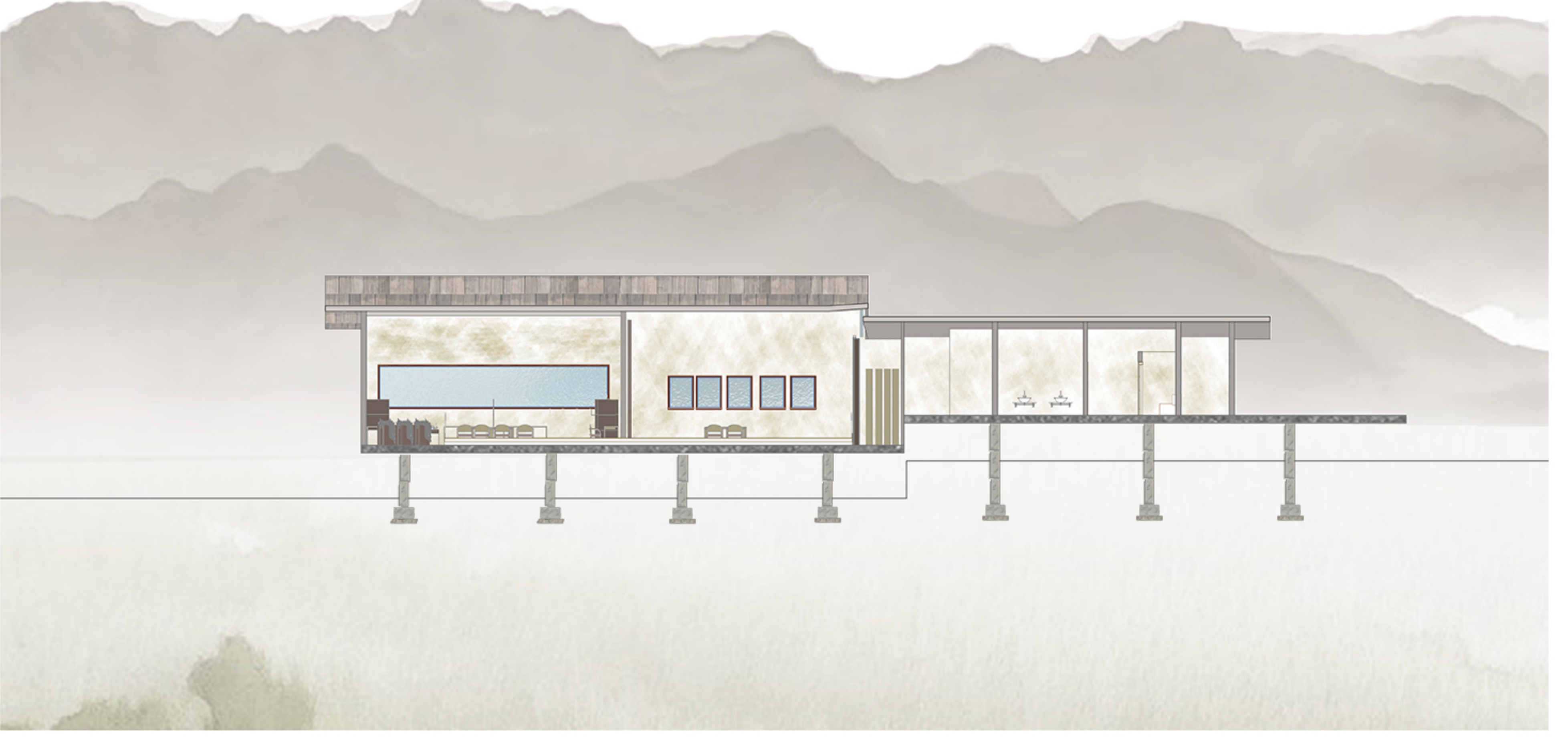
SECOND SECTION 1/50
