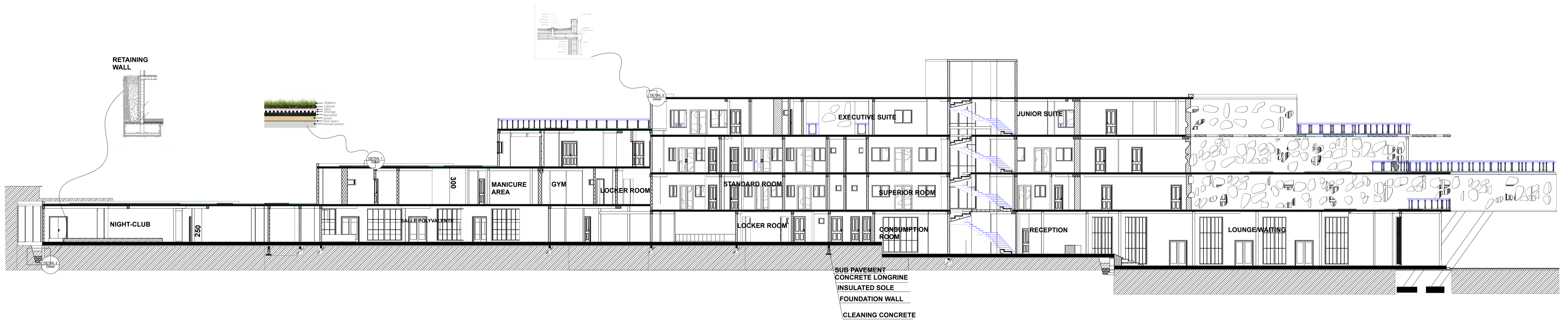
SECTION AA'
