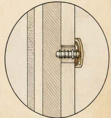
DETAIL C STRUCTURAL JOINT
