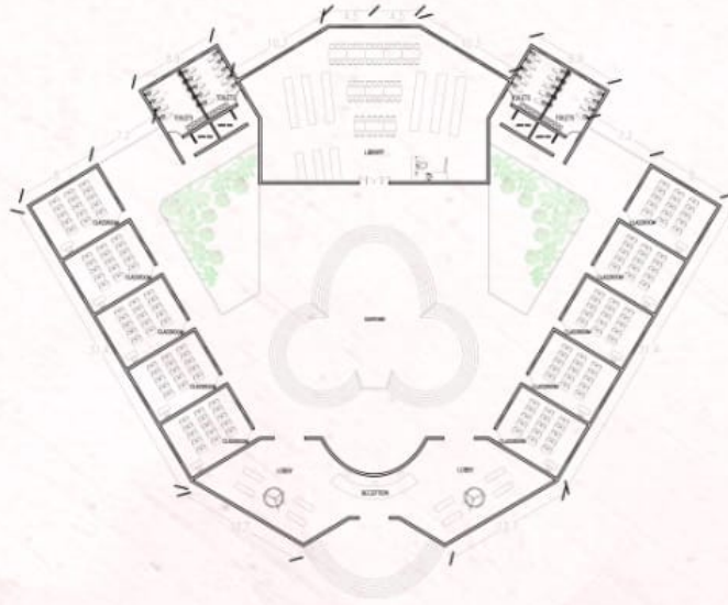
GROUND FLOOR PLAN SCALE - 1 : 200
