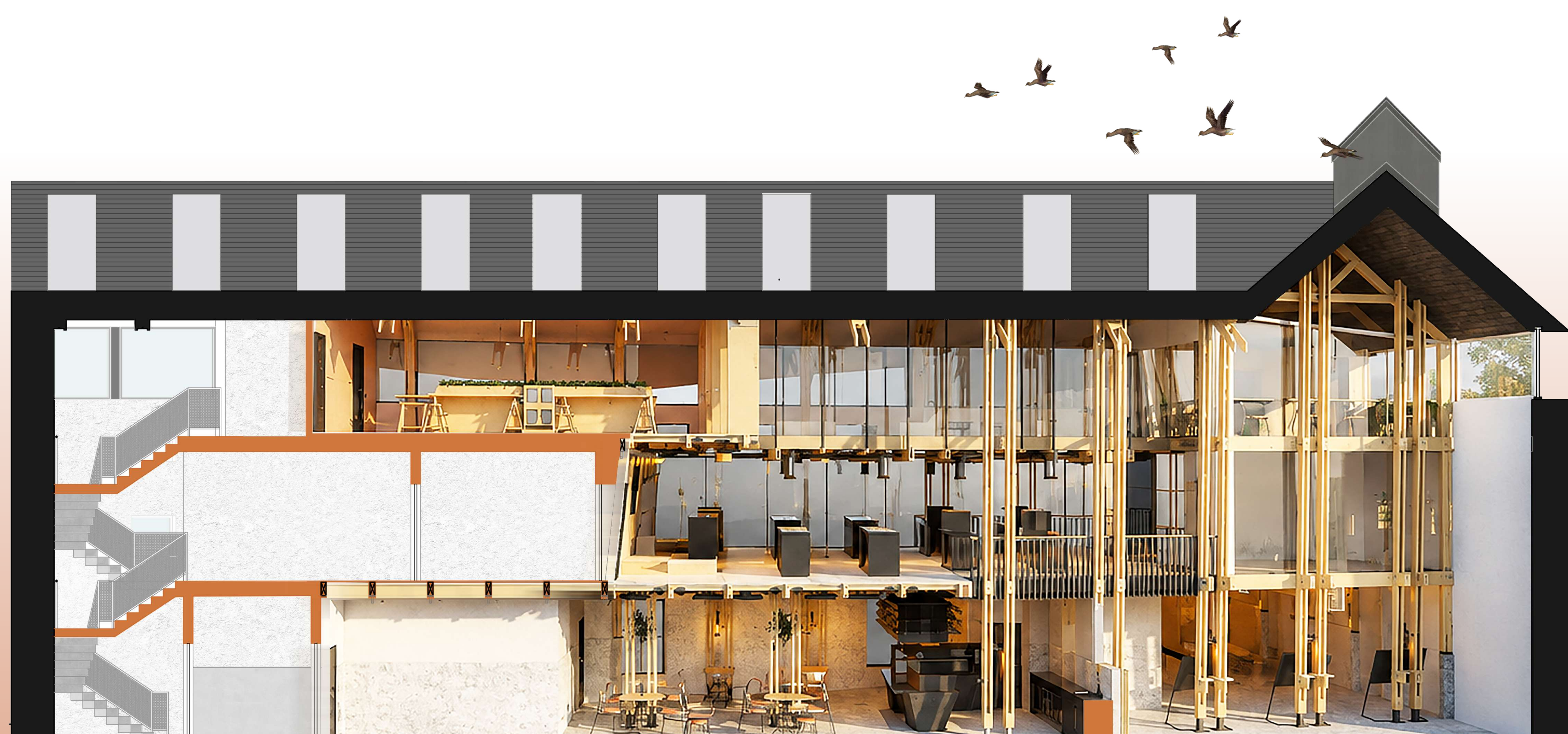
SECTIONAL PERSPECTIVE
