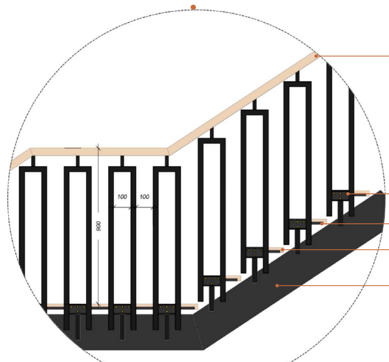
BALAUSTRADE DETAIL OF PART K STAIRS
