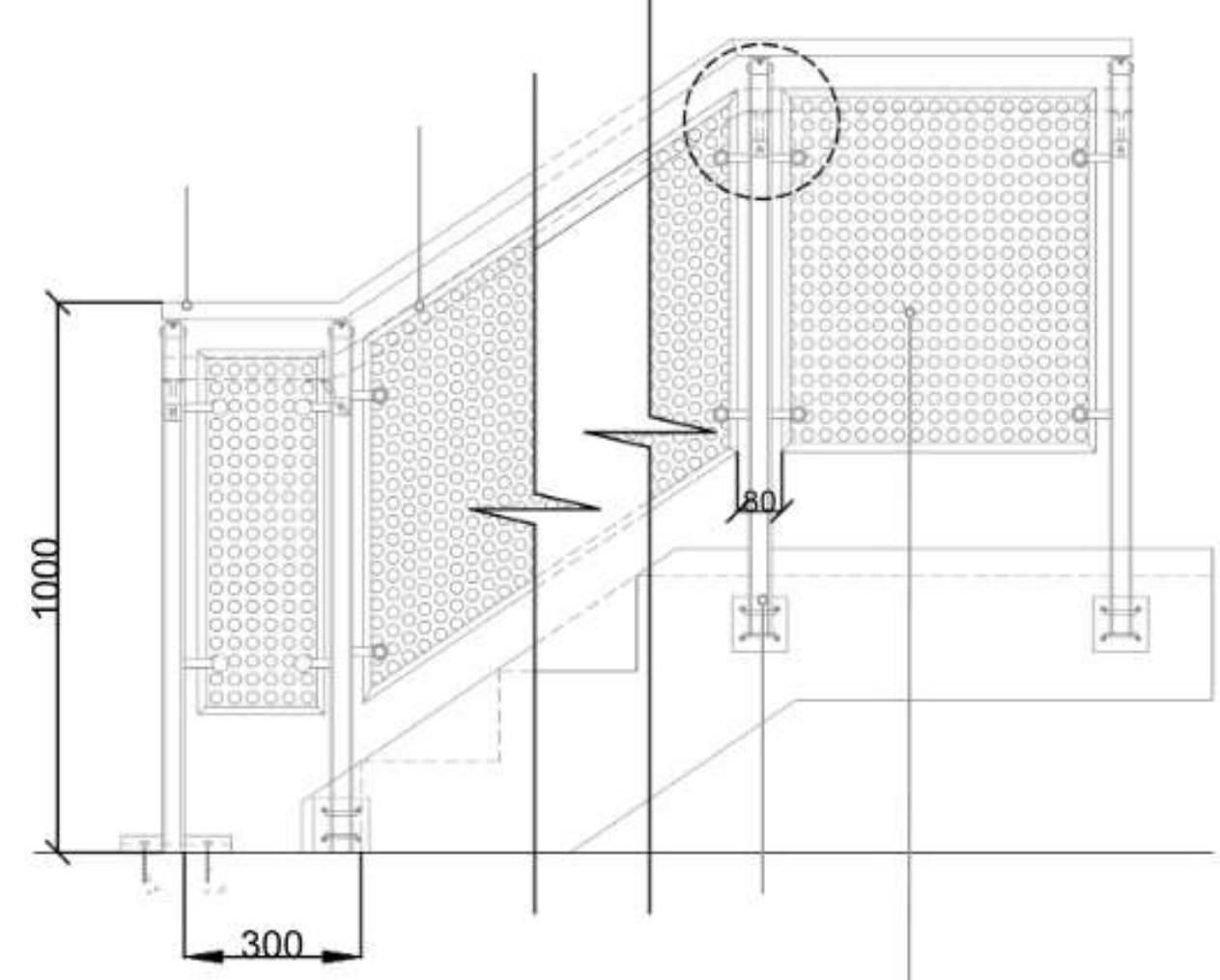
FIRE STAIR CORE B HANDRAIL DETAIL
