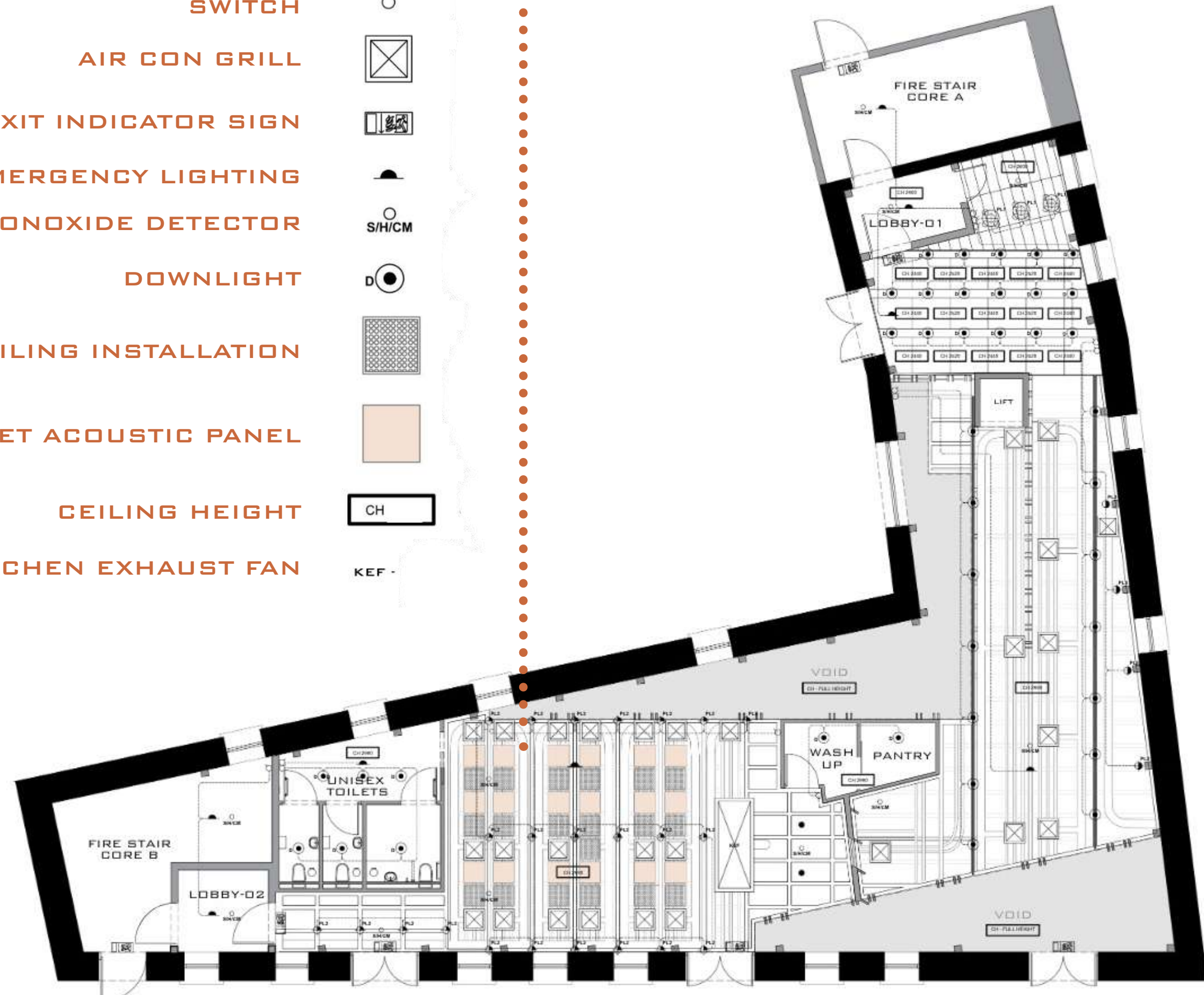
REFLECTIVE CEILING PLAN
