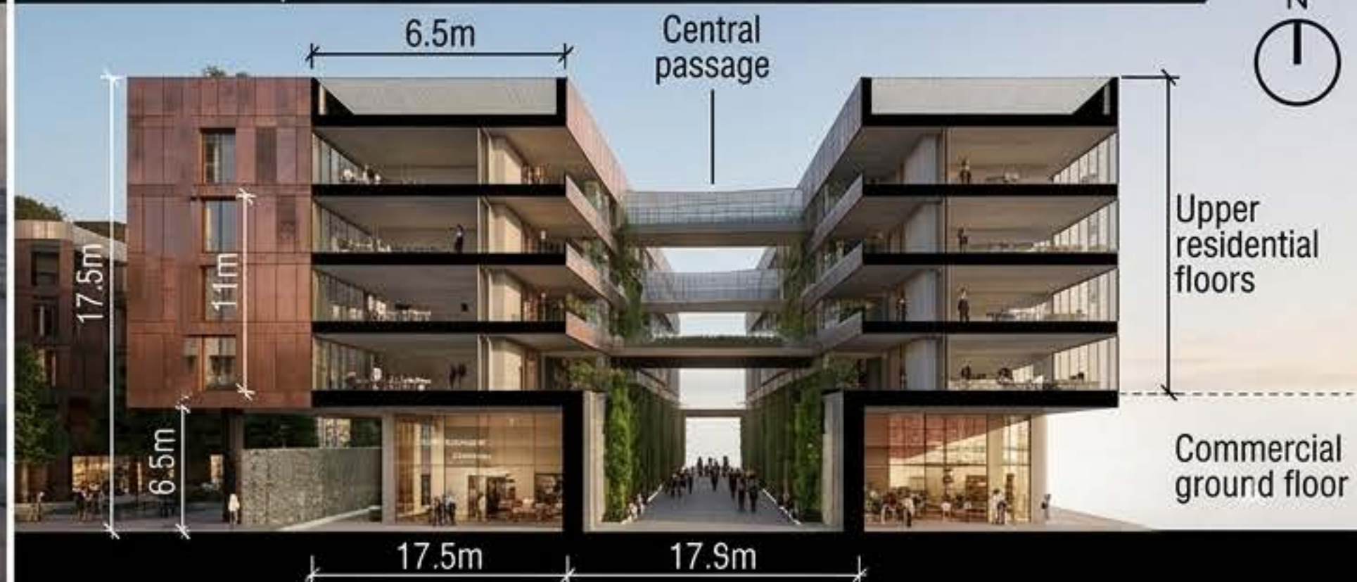
Architectural Solution Close-up - Mixed-Use Building Perspective Section
