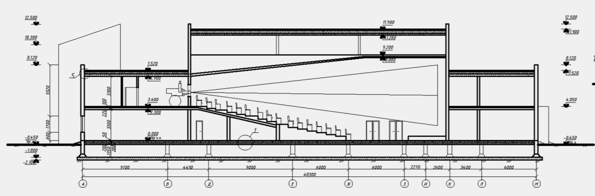
Incision 1-1
