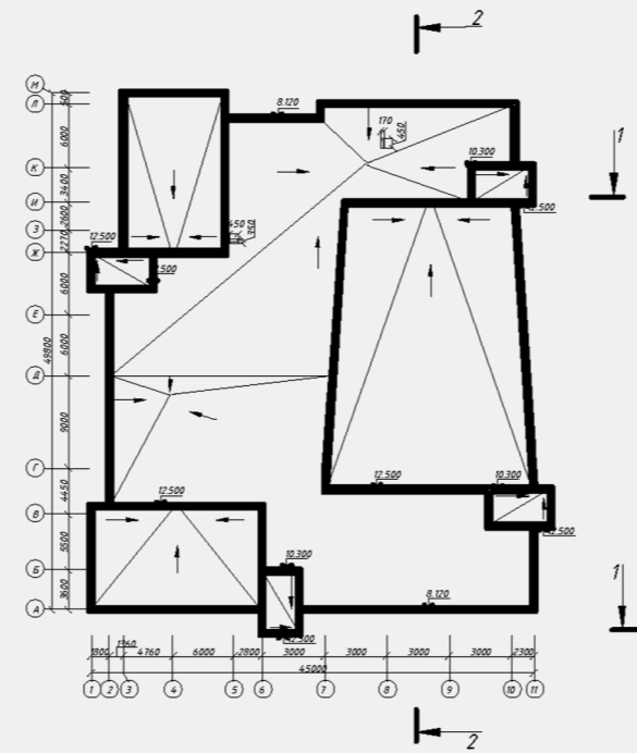
Roofing plan
