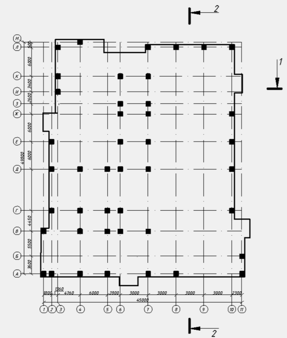
Foundation plan
