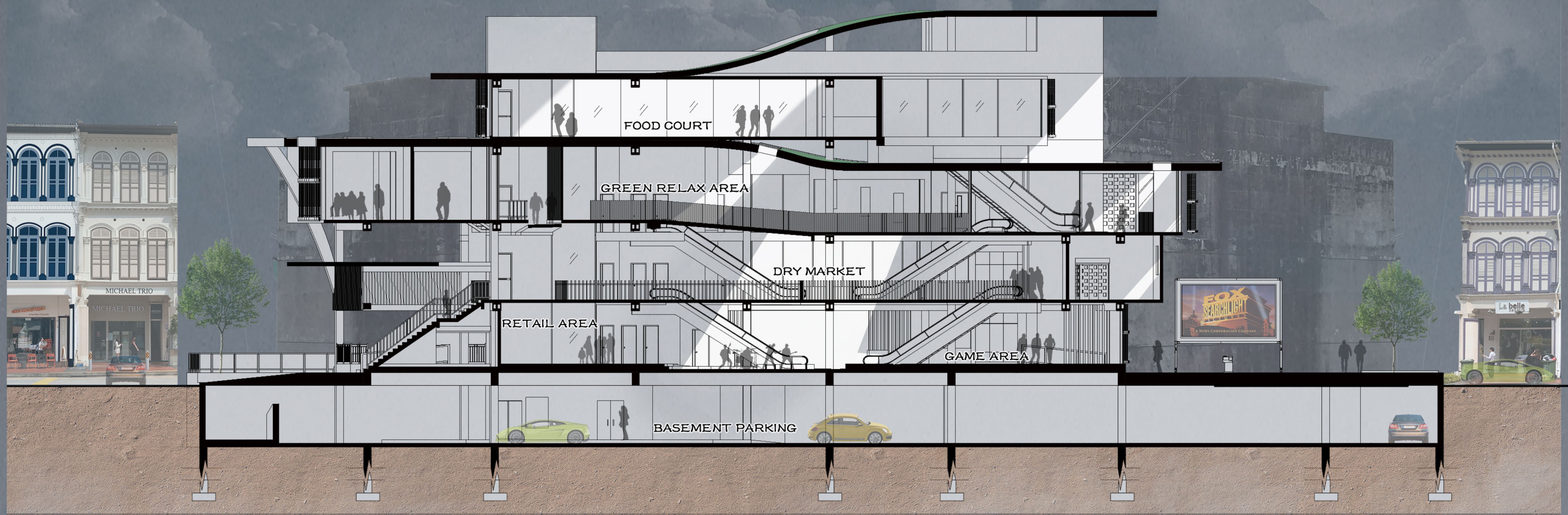
SECTION A- A SCALE 1:100
