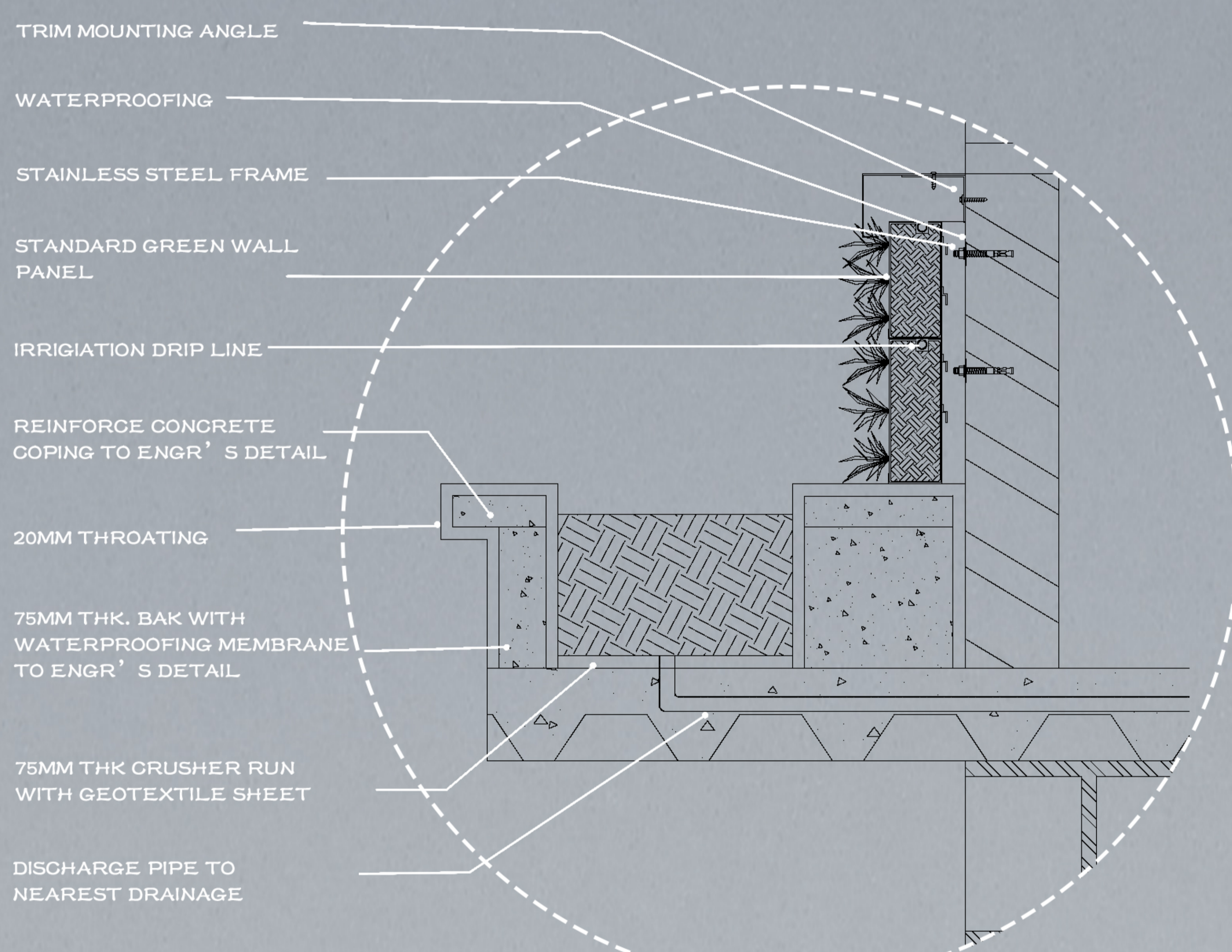
DETAIL SECTION 2 SCALE 1:5
