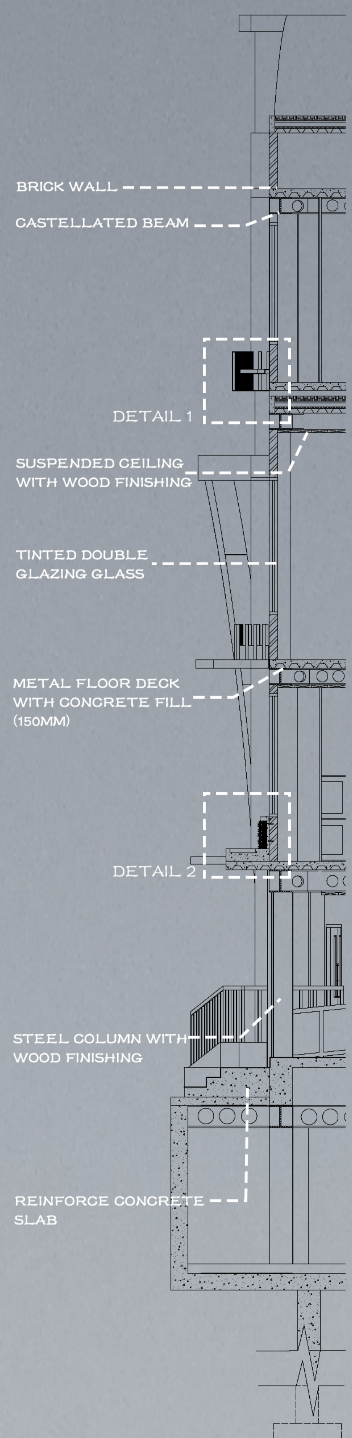
TYPICAL SECTION SCALE 1:40
