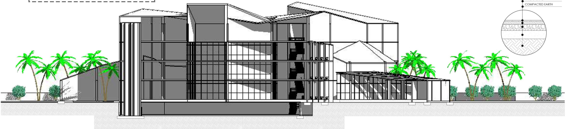
SECTIONAL ELEVATION AT DD'
