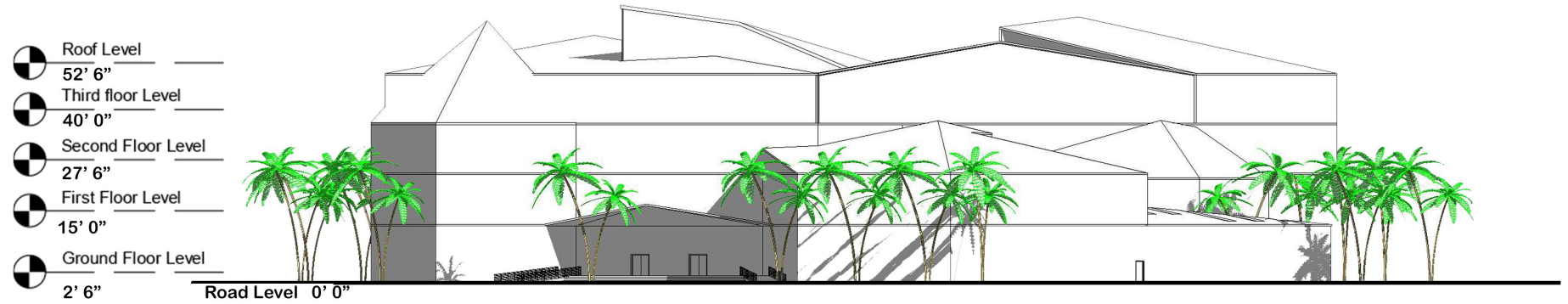
SOUTH ELEVATION
