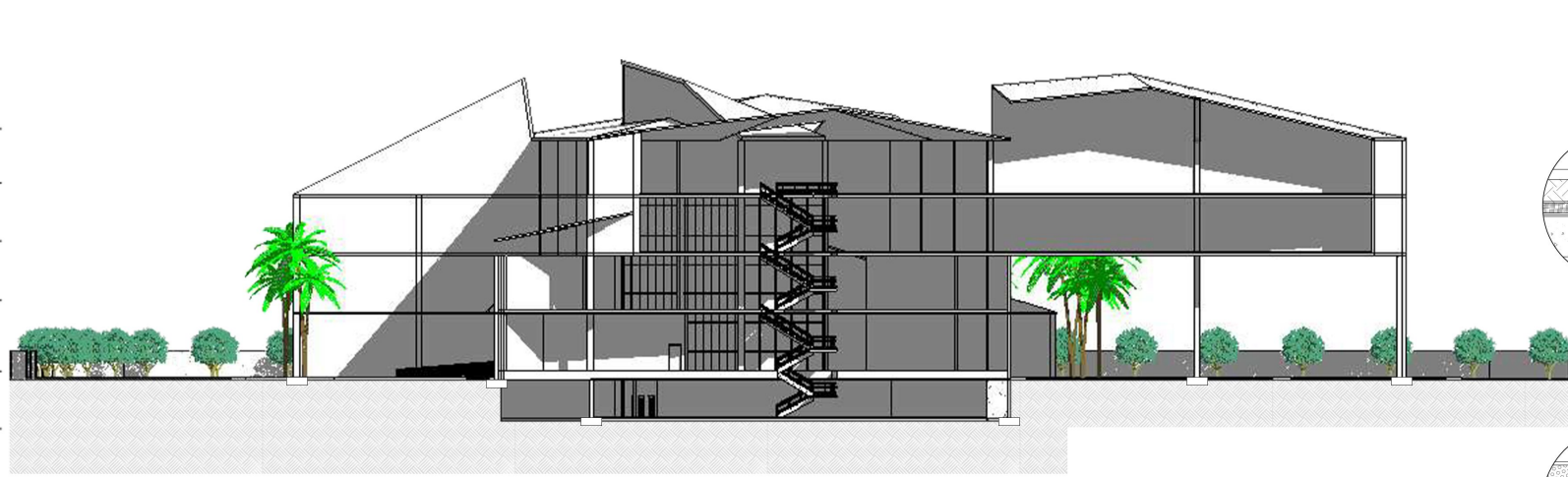
SECTIONAL ELEVATION AT AA'
