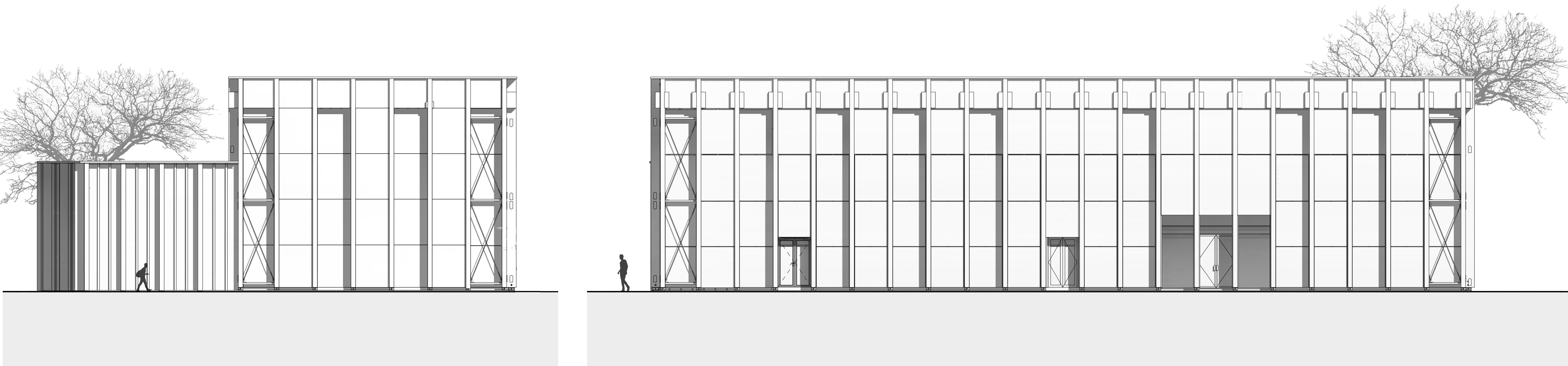
West Facade
