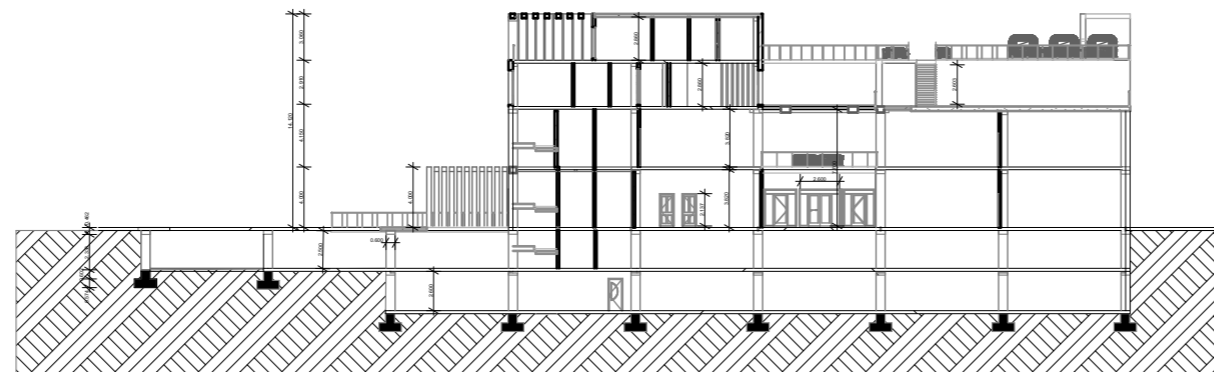
SECTION 2-2
