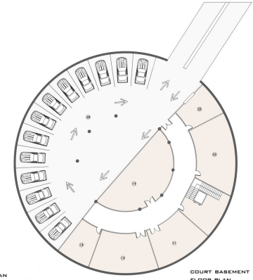
COURT BASEMENT FLOOR PLAN
