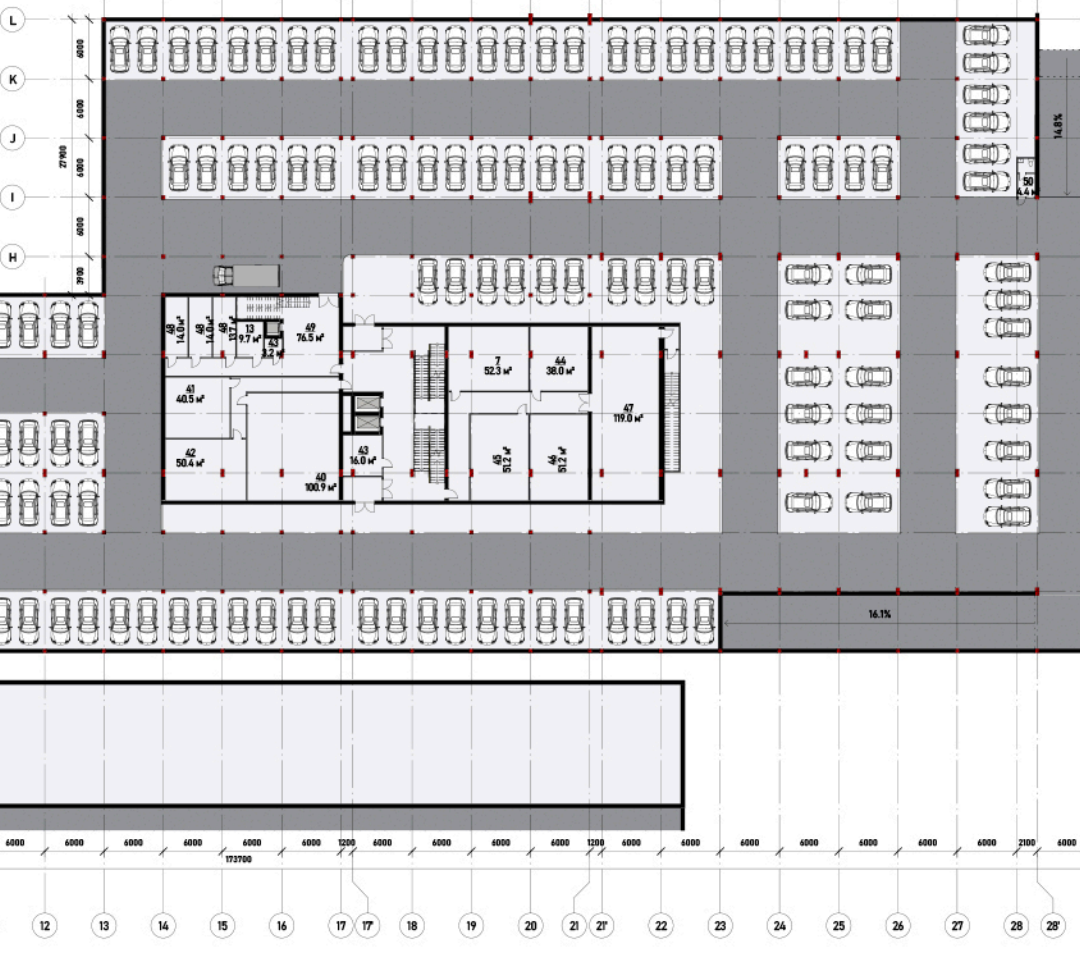
LEVEL 3 PLAN
