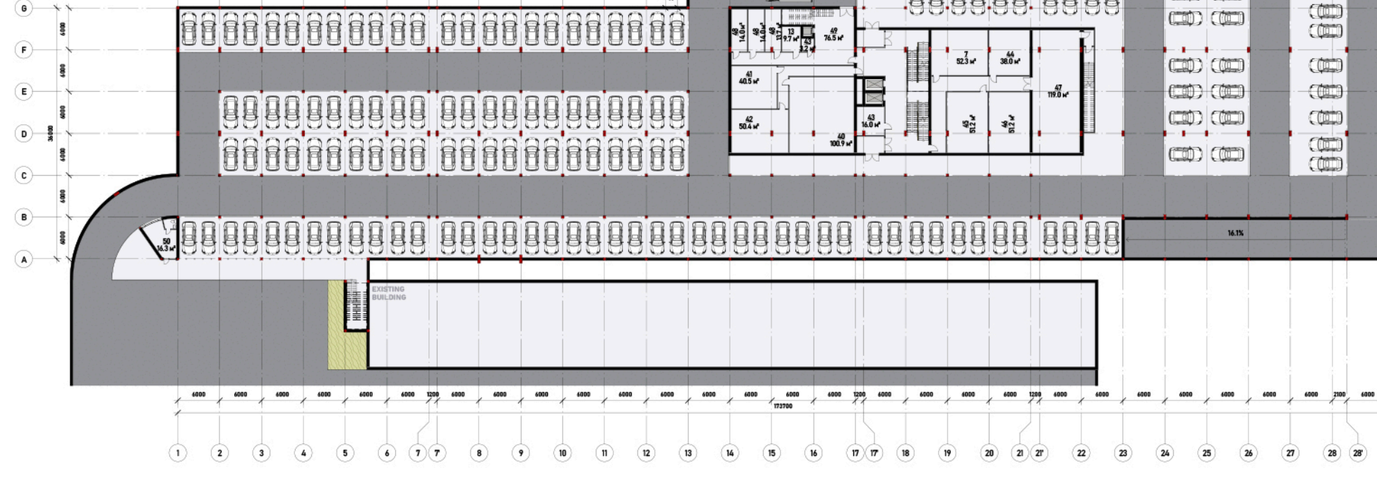
LEVEL -1 PLAN
