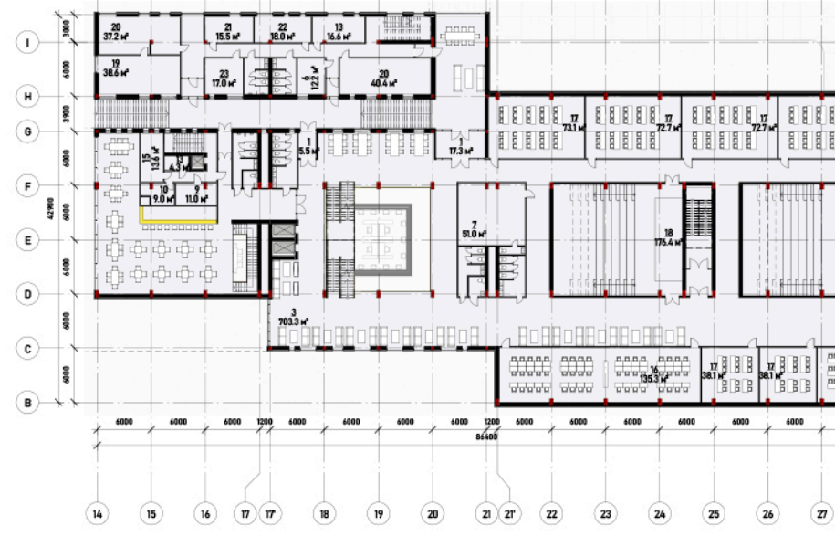
LEVEL 2 PLAN
