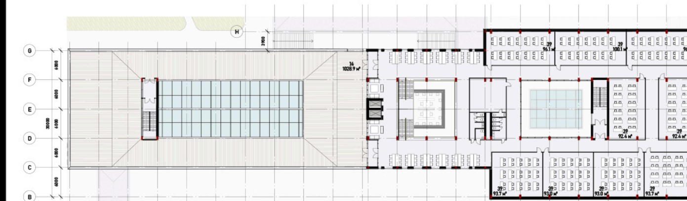
LEVEL 6 PLAN
