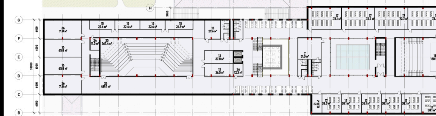
LEVEL 5 PLAN
