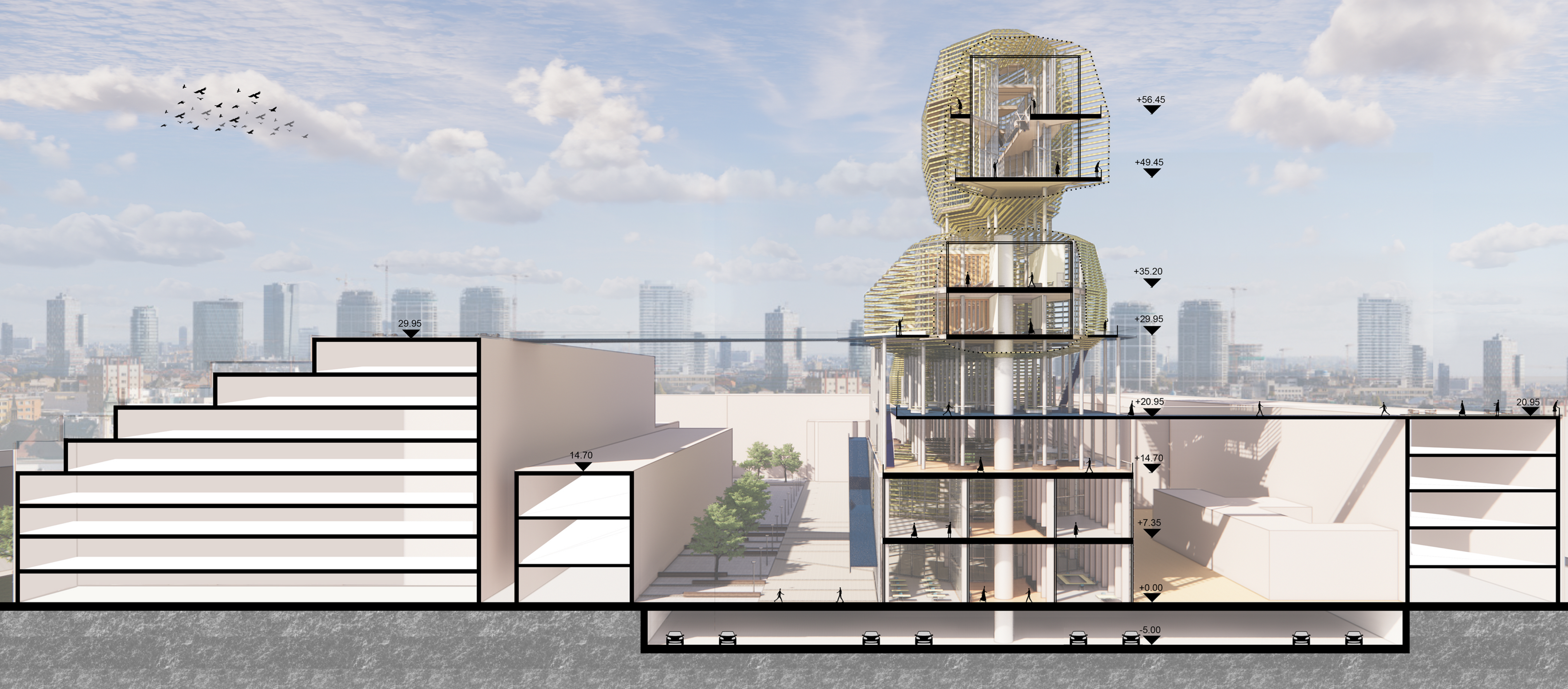
Section B-B 1:250
