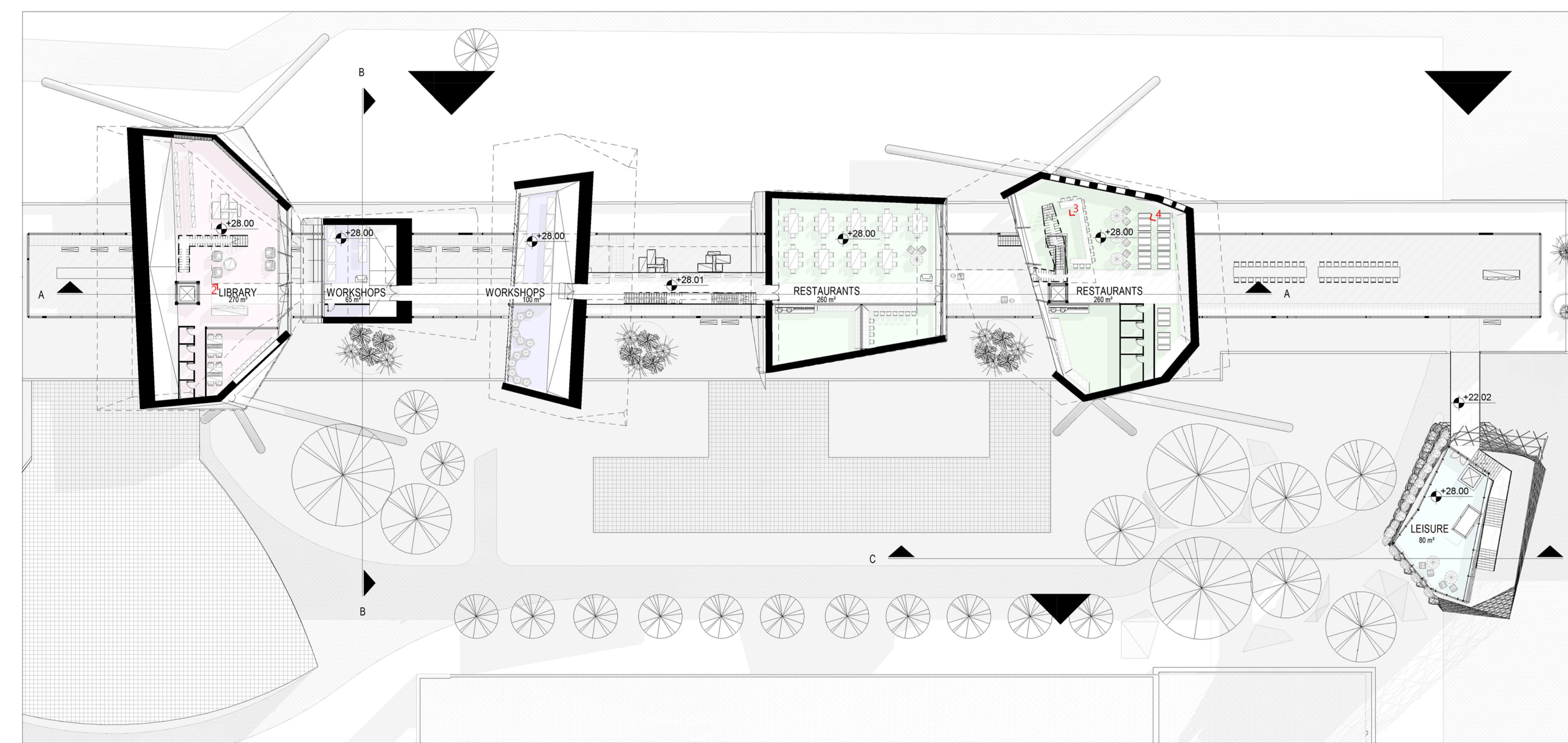
FIRST FLOOR 1:250
