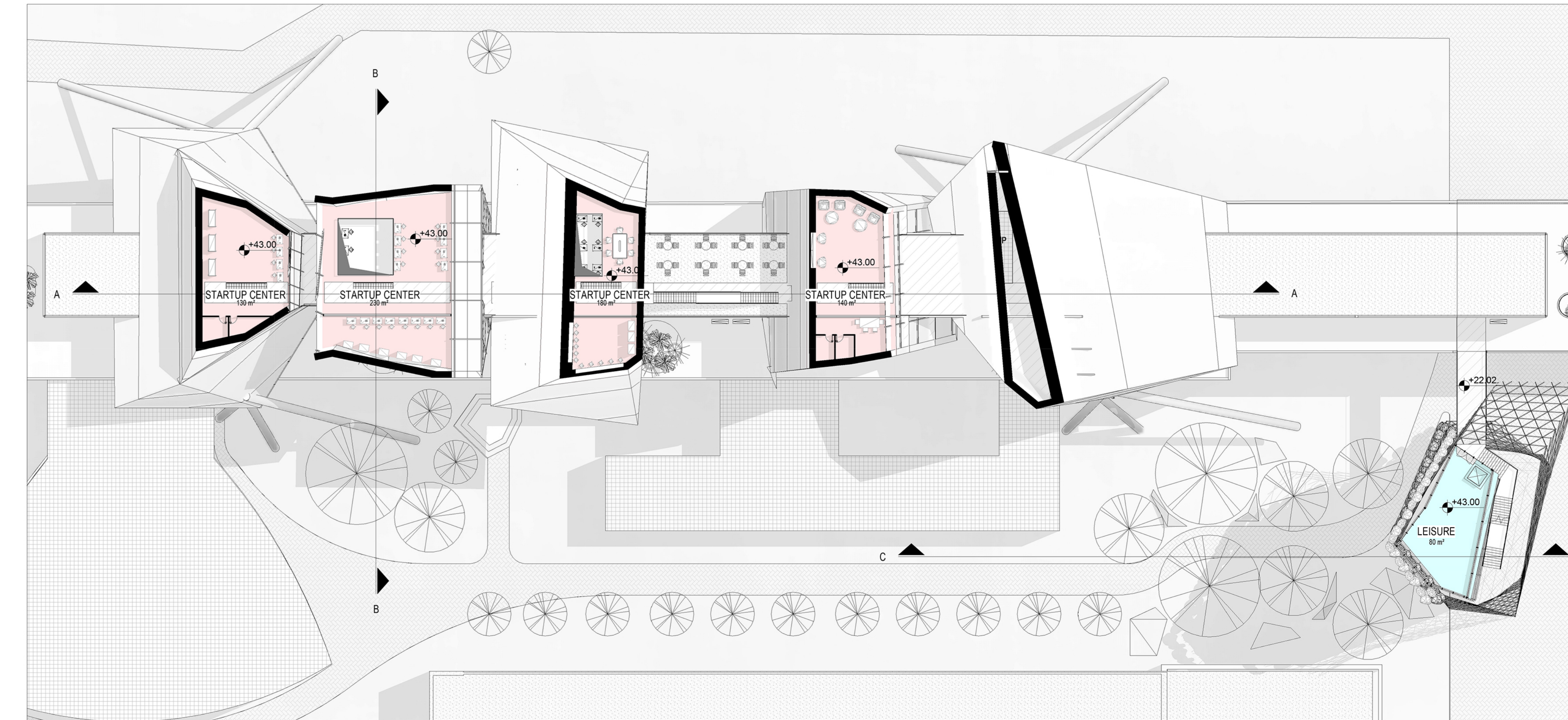
FOURTH FLOOR 1:250
