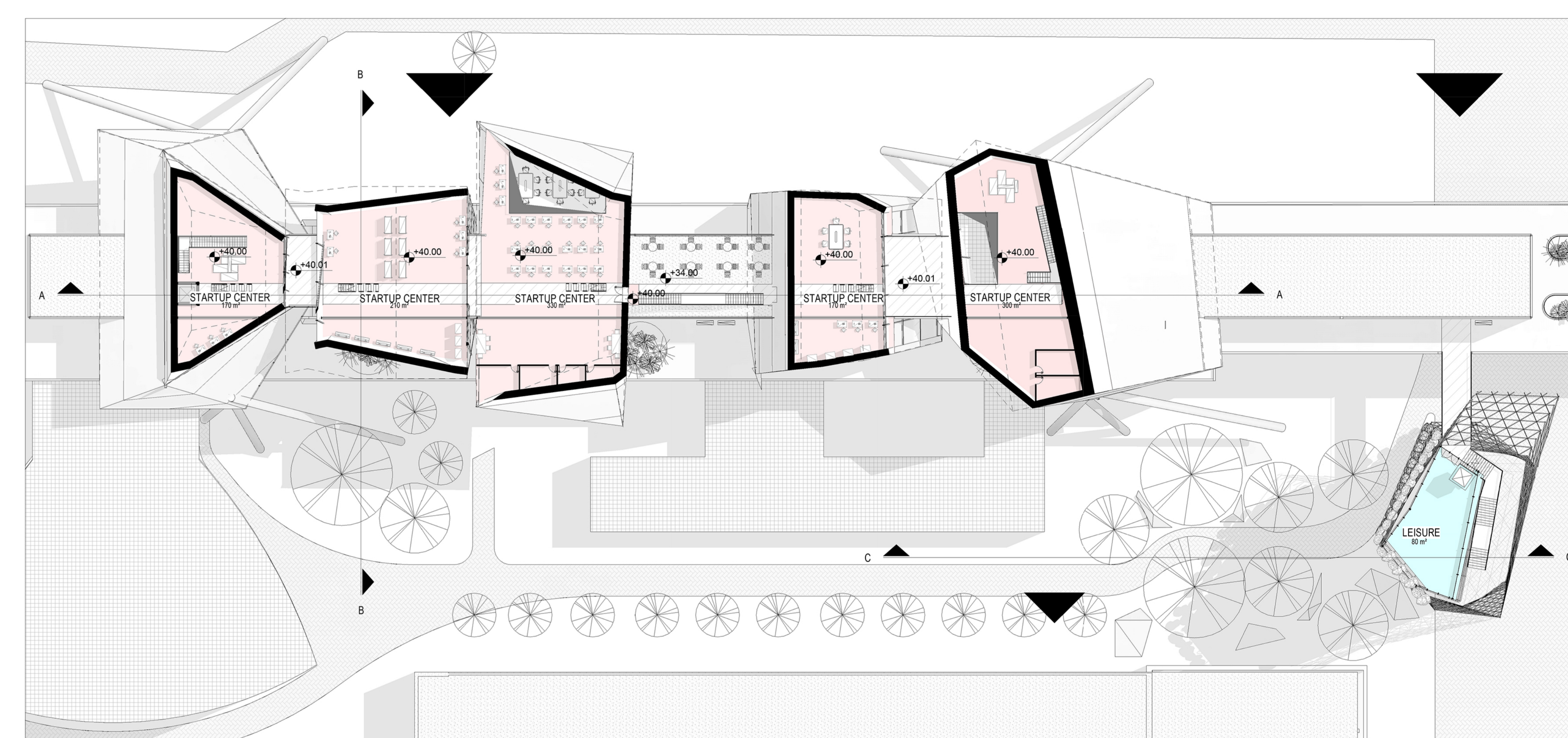
THIRD FLOOR 1:250
