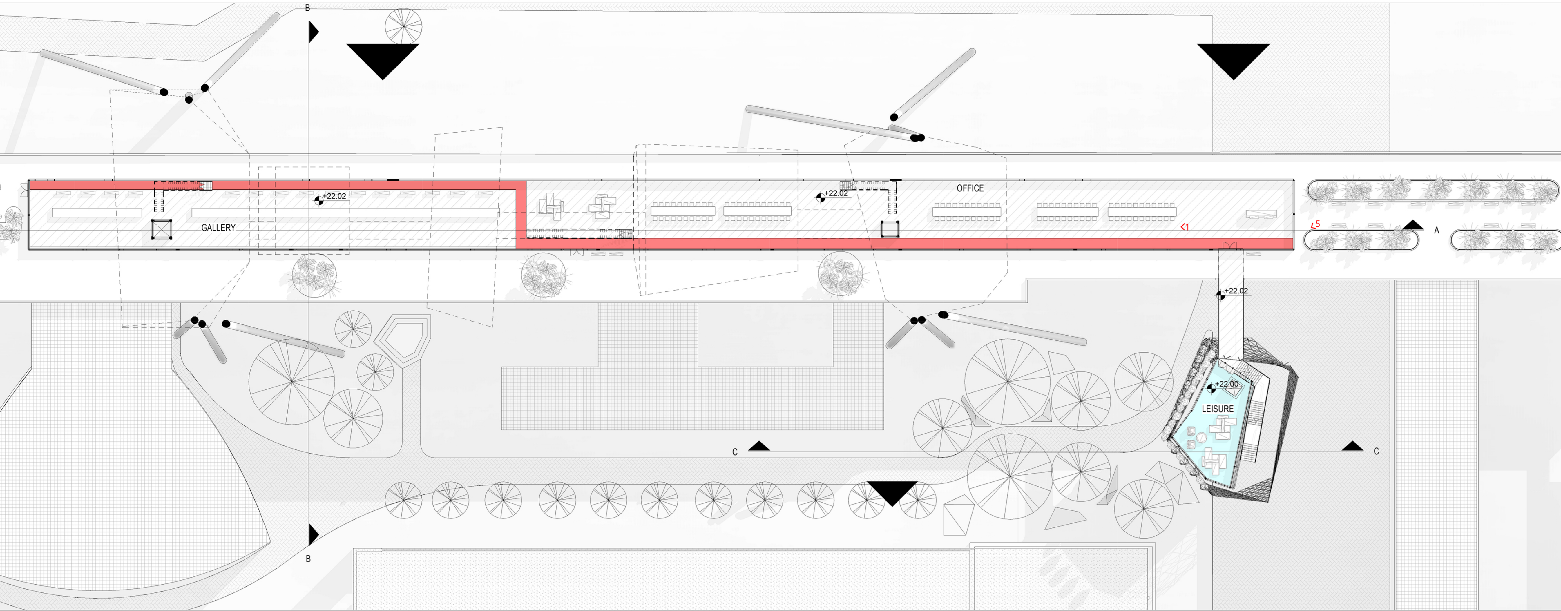
GROUND FLOOR 1:250
