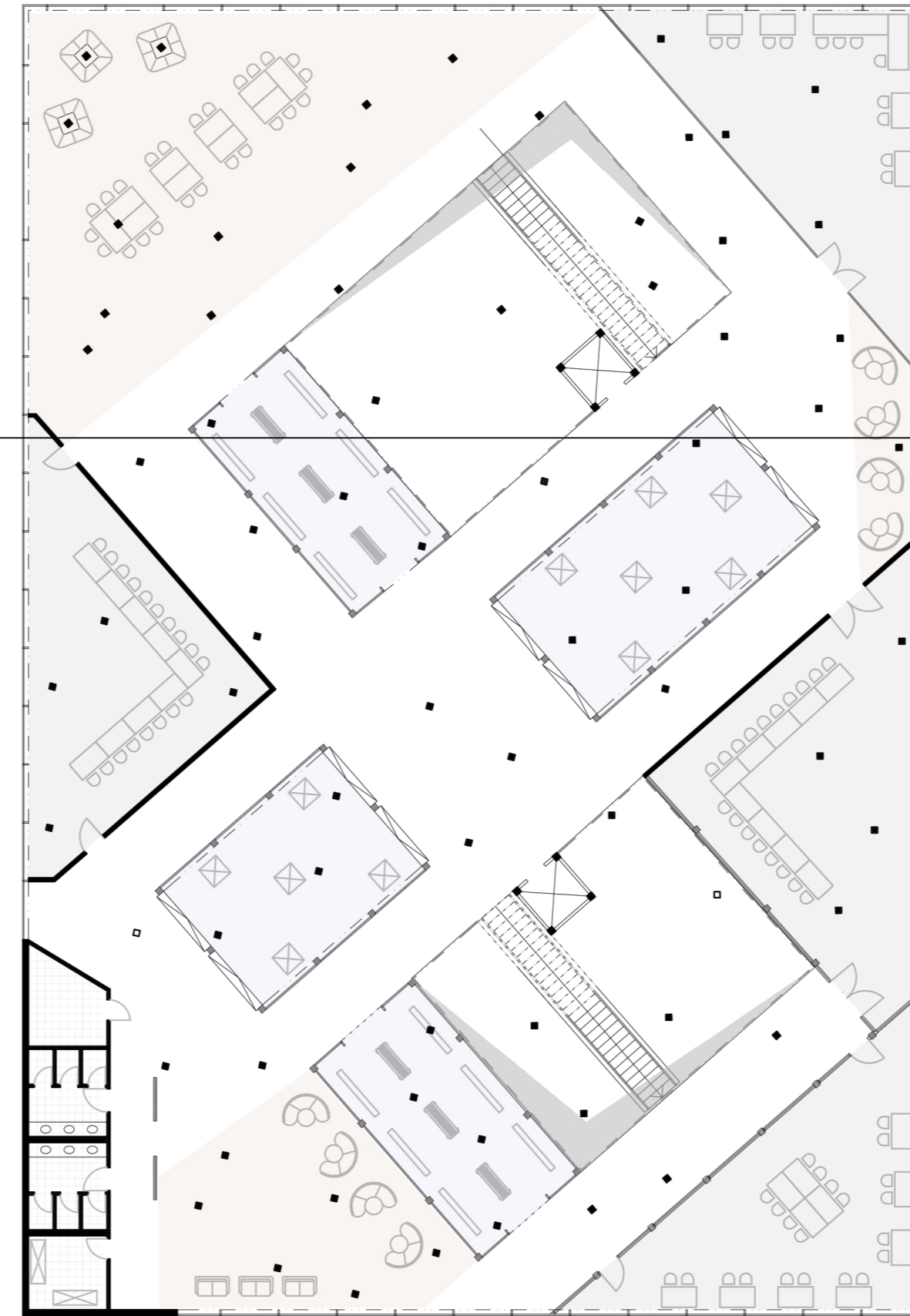
First Floor 1:200 Open space & Leisure Classes Show rooms
