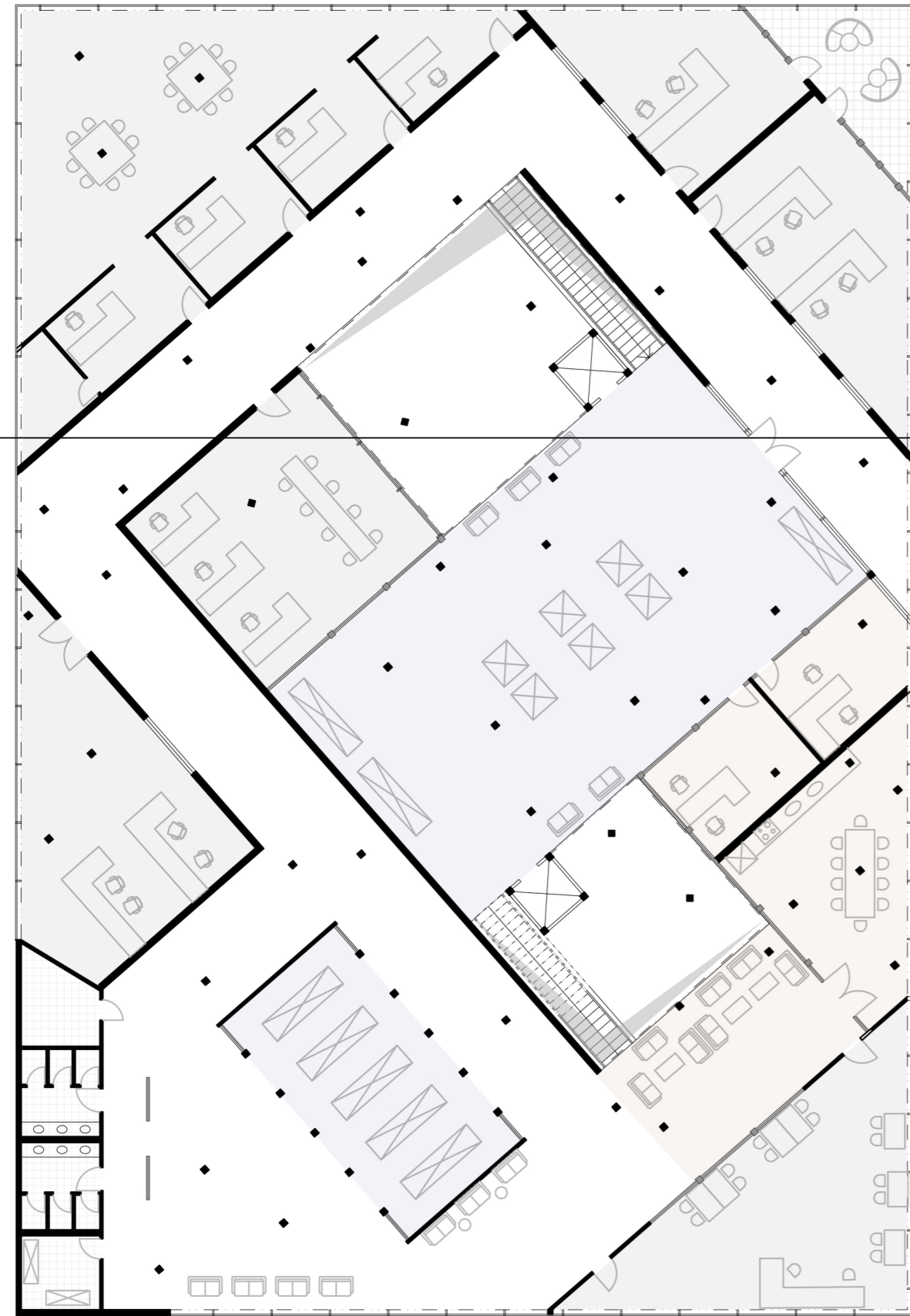
Second Floor 1:200 Office & Staff Laboratories & research Library & showcase
