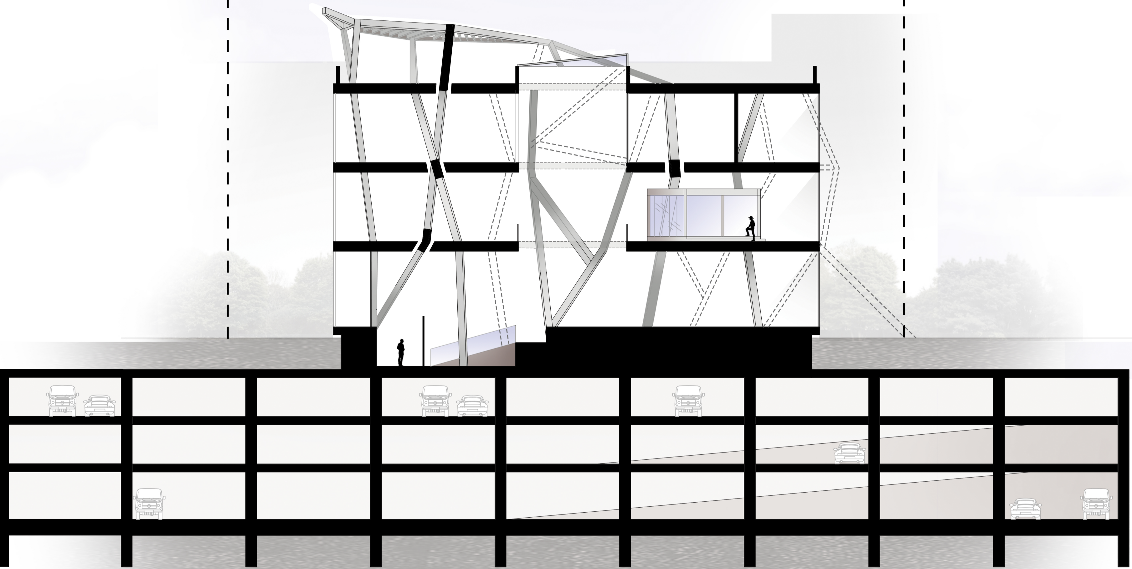
Section E - Innovation center 1:100
