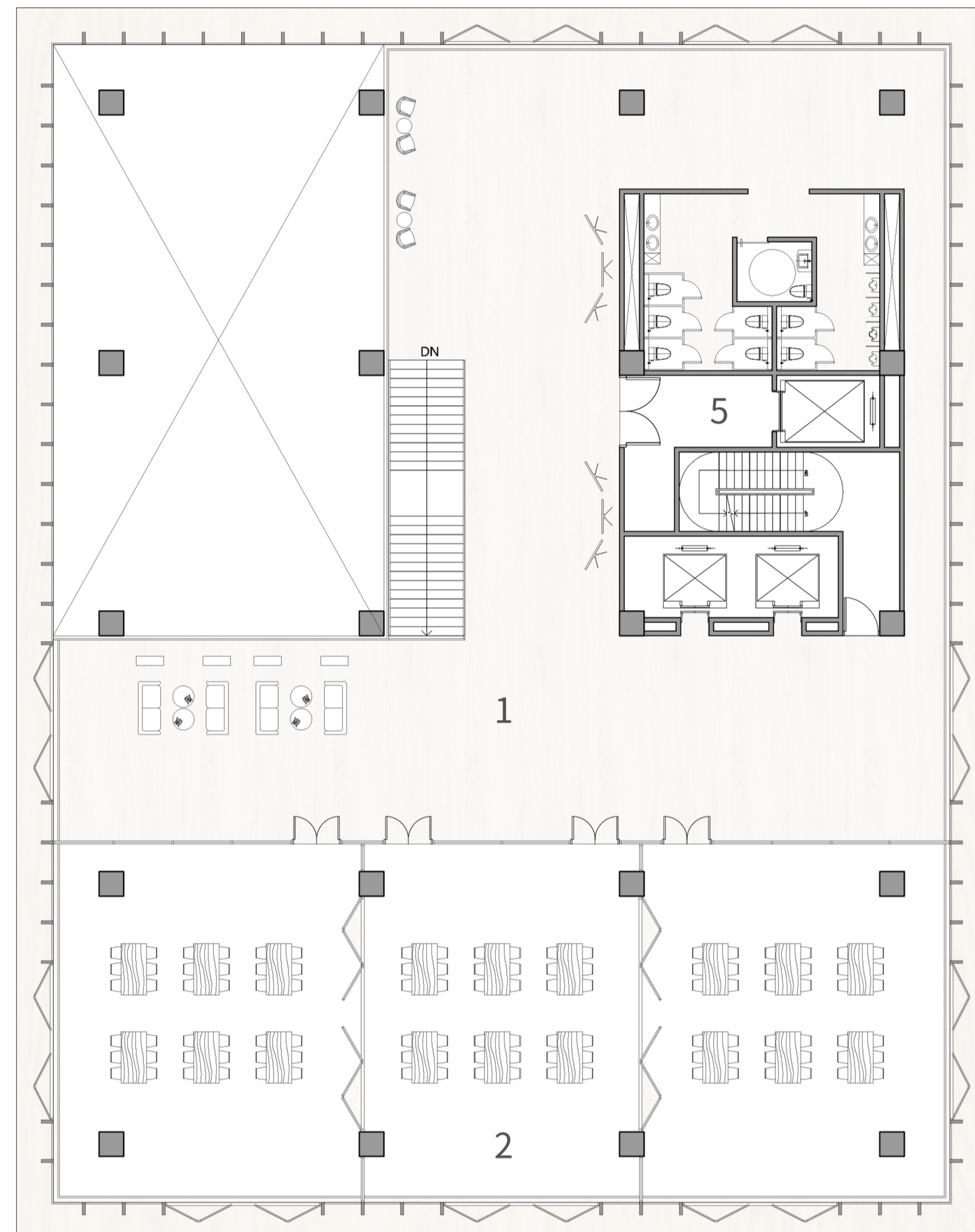
A-1F Plan Scale:1/200 ☹
