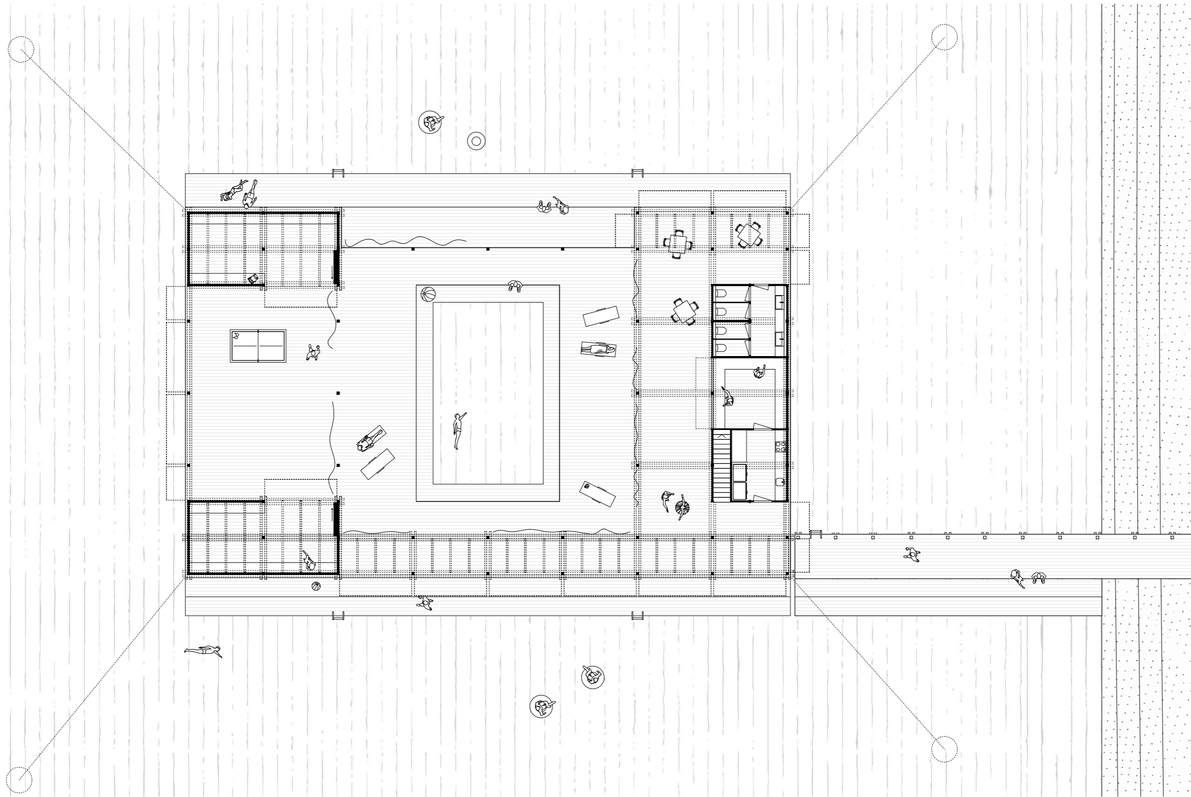
ground floor public bath | 1:200
