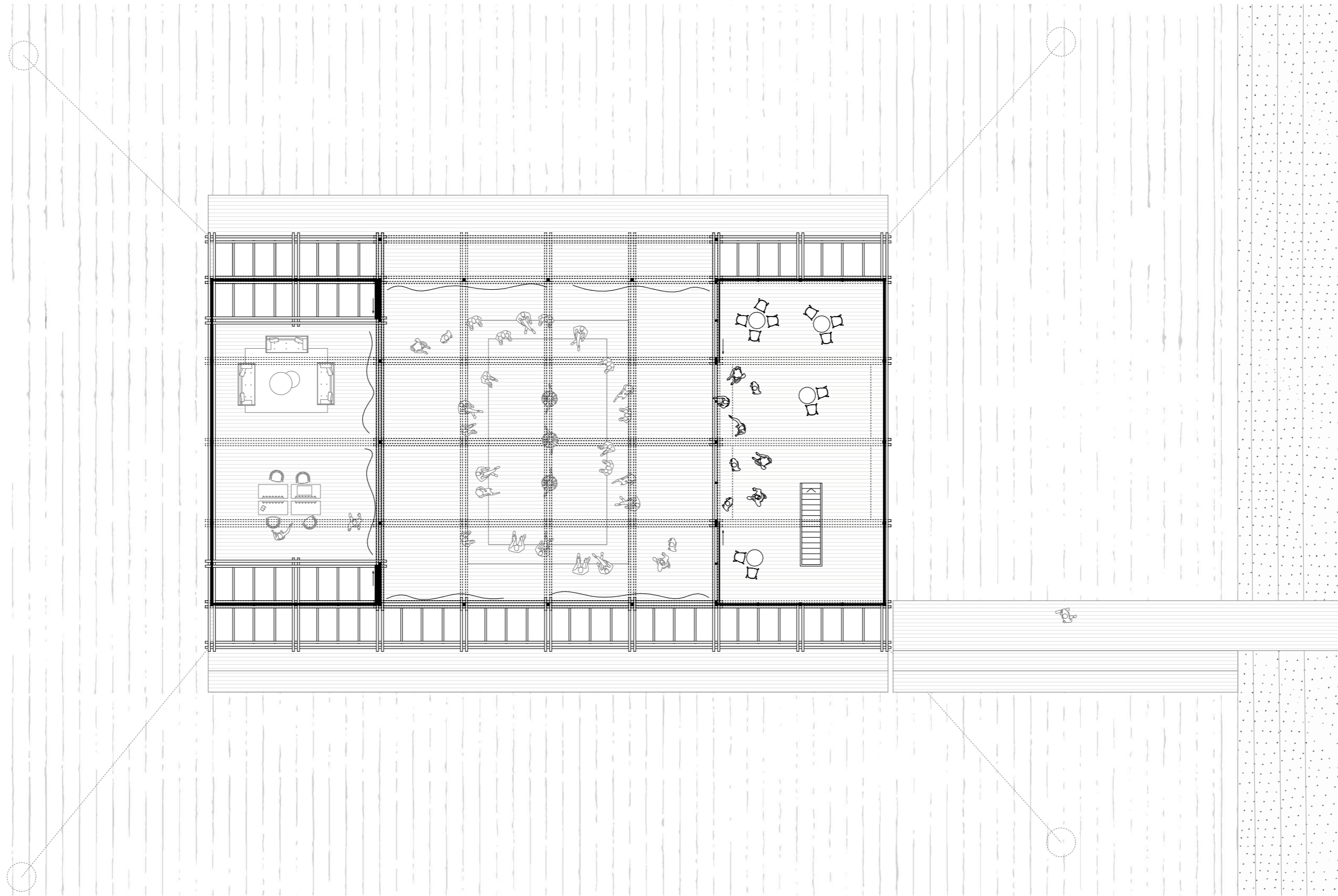
floor plan upper level theatre | 1:200
