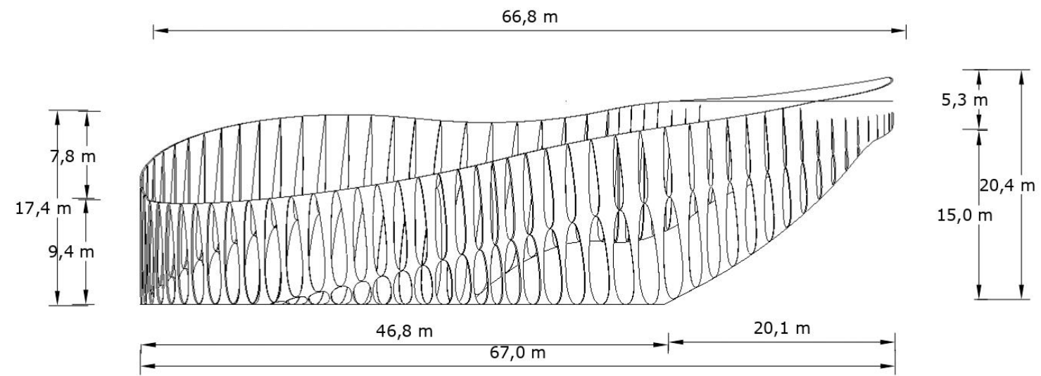
TAMPAK B SECOND SKIN skala 1:400
