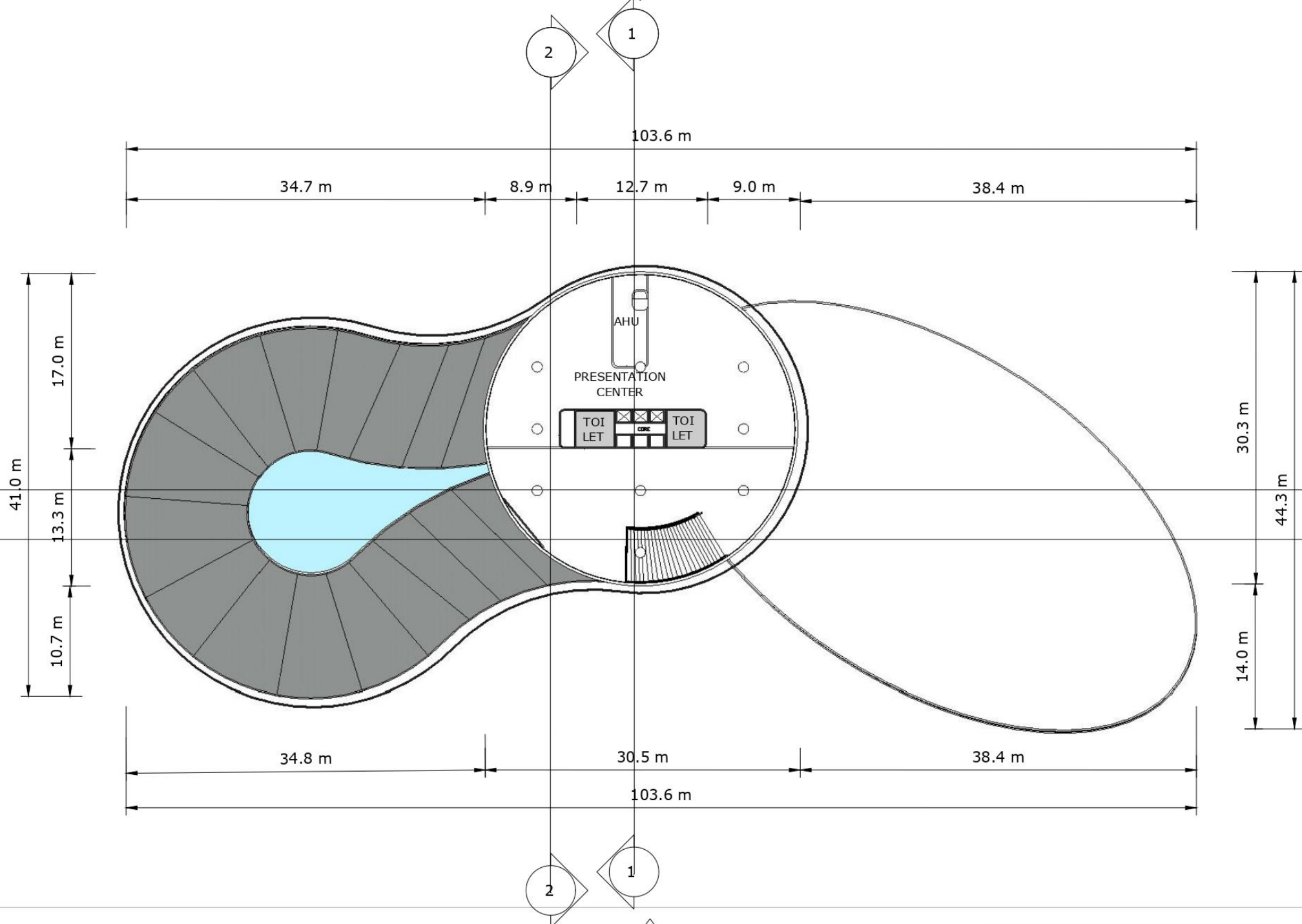
DENAH LT 5 skala 1:400
