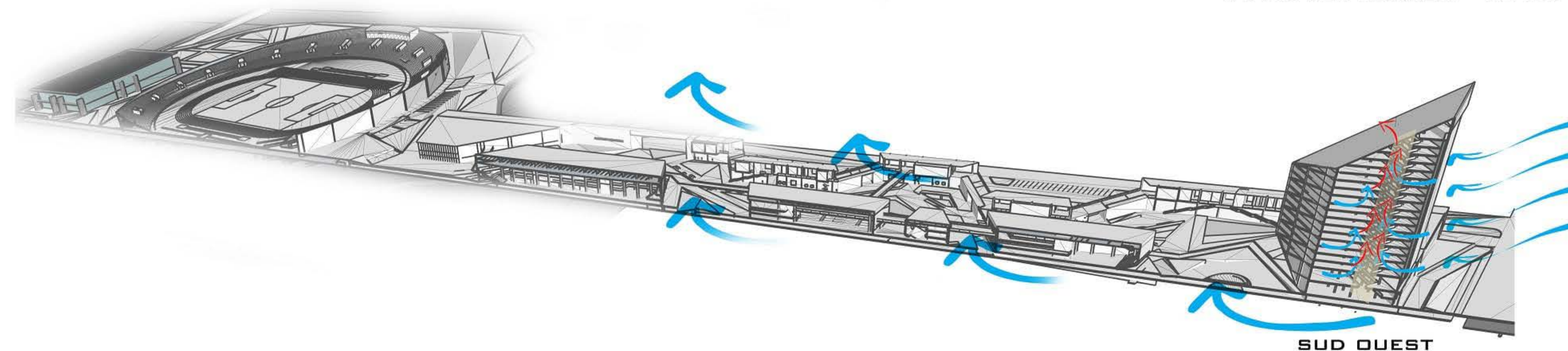
STACK VENTILATION - HOTEL
