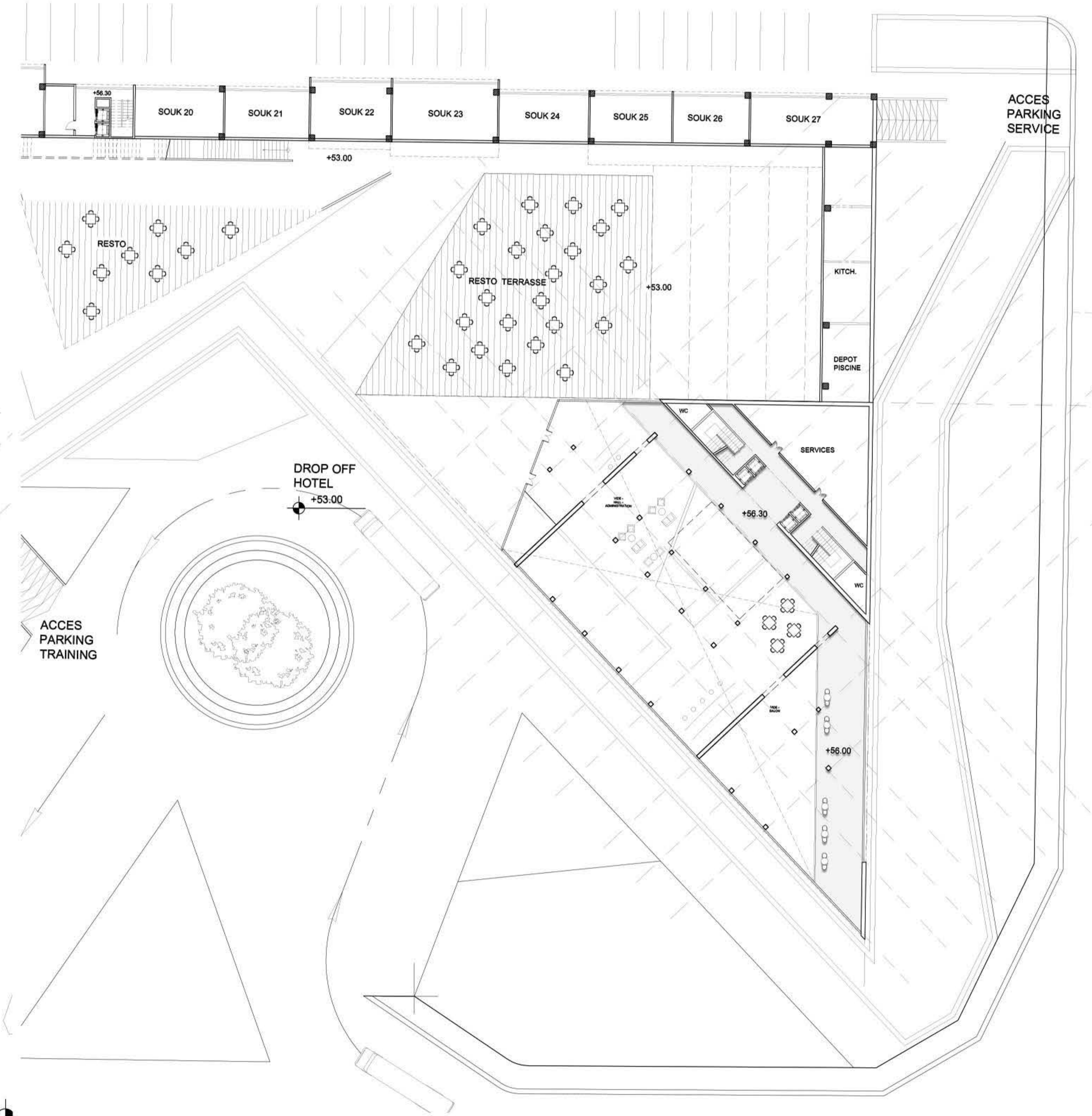
PLAN MEZANINE
