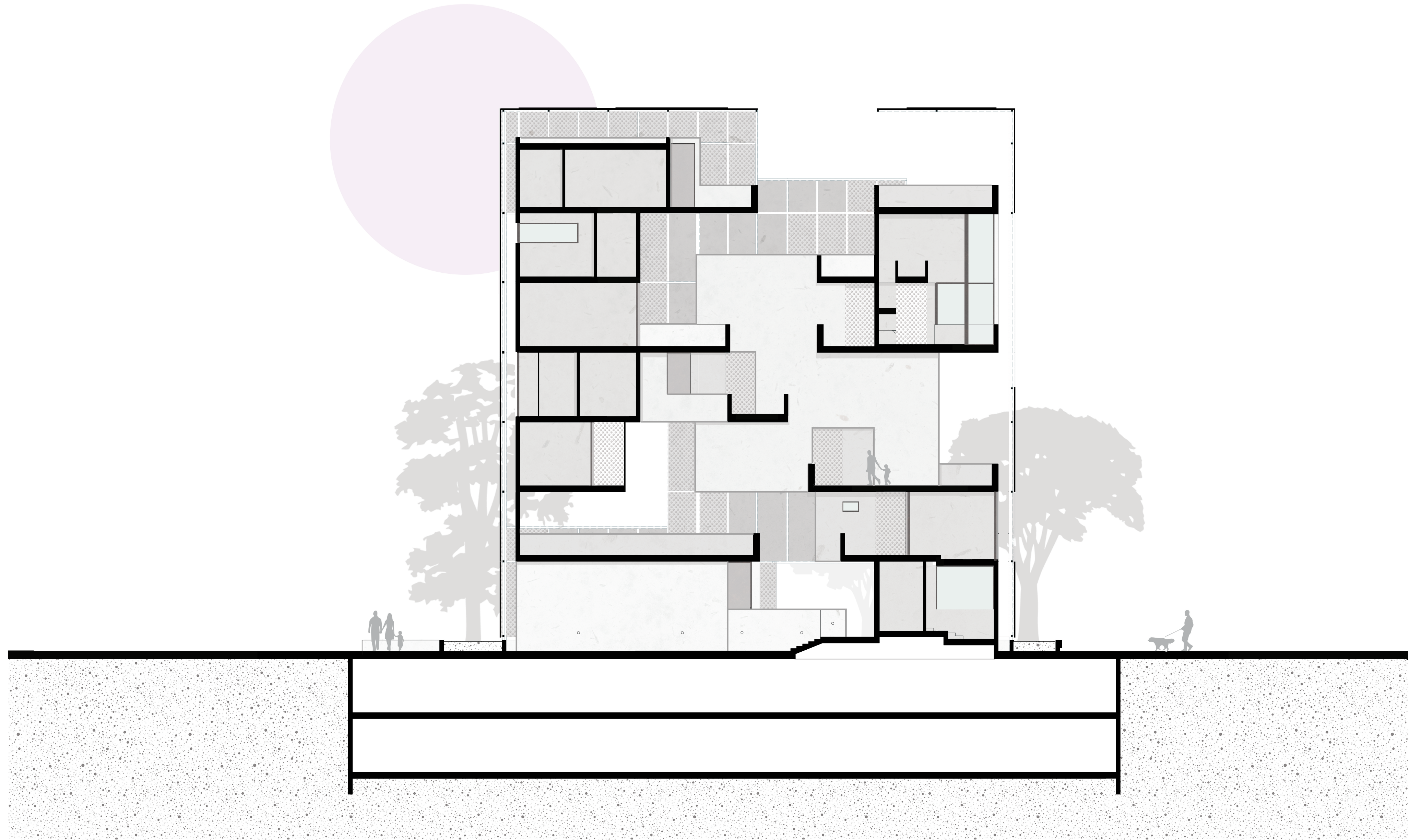
Section AA
