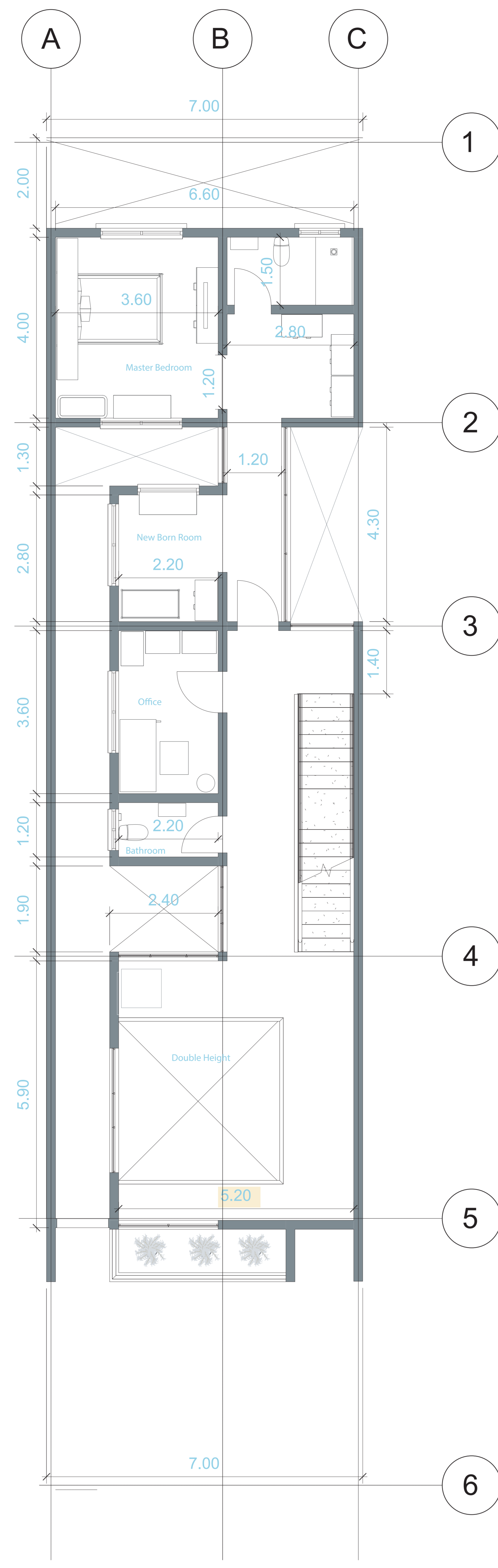
First Floor Scale 1/50
