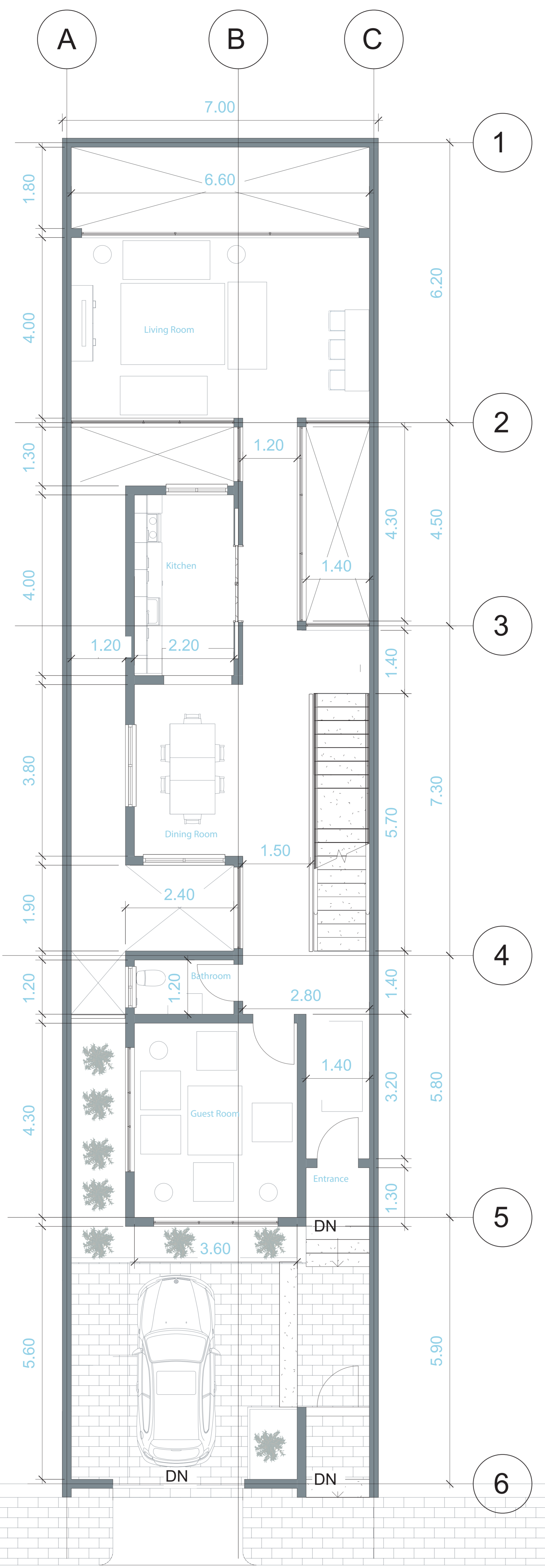
Ground Floor Scale 1/50
