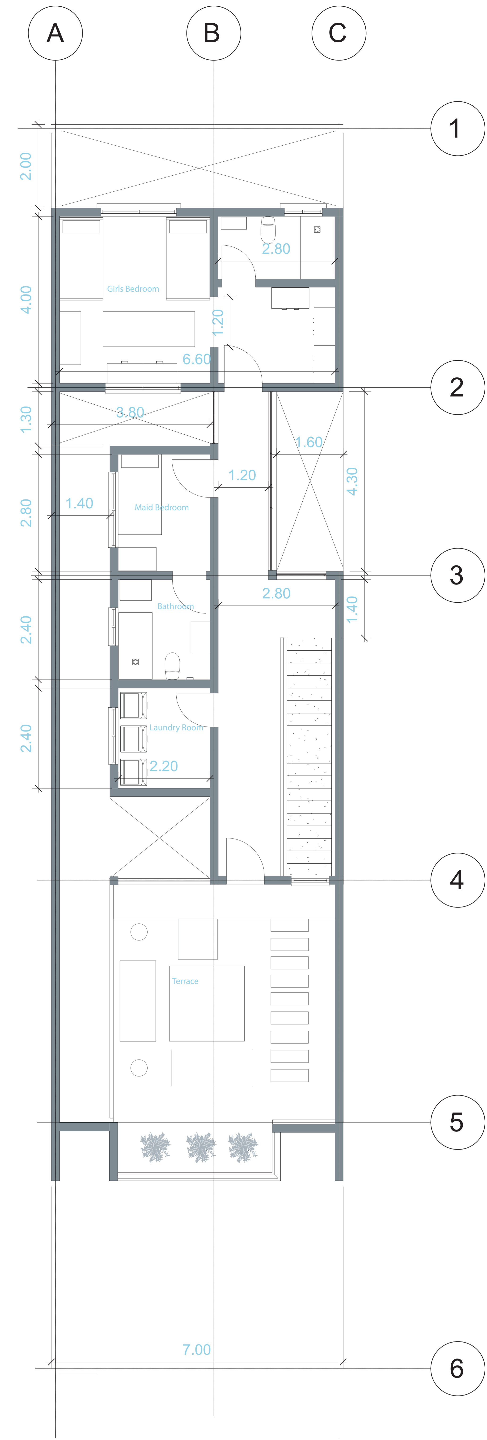
Second Floor Scale 1/50
