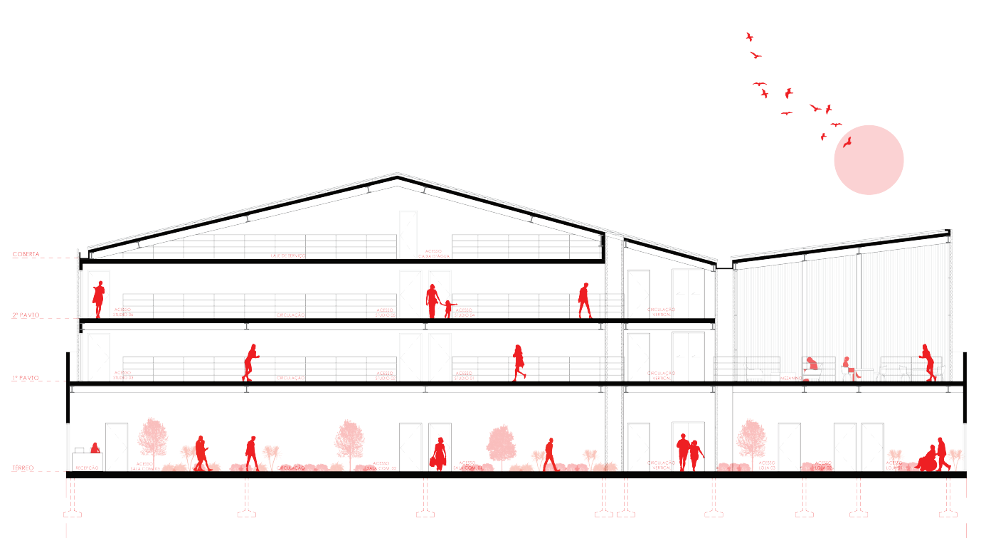
SECTION BB'
