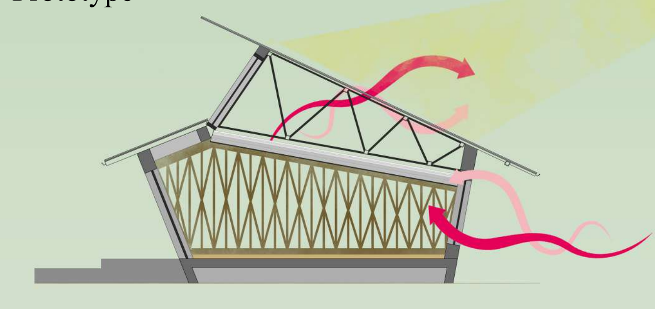
Section A
