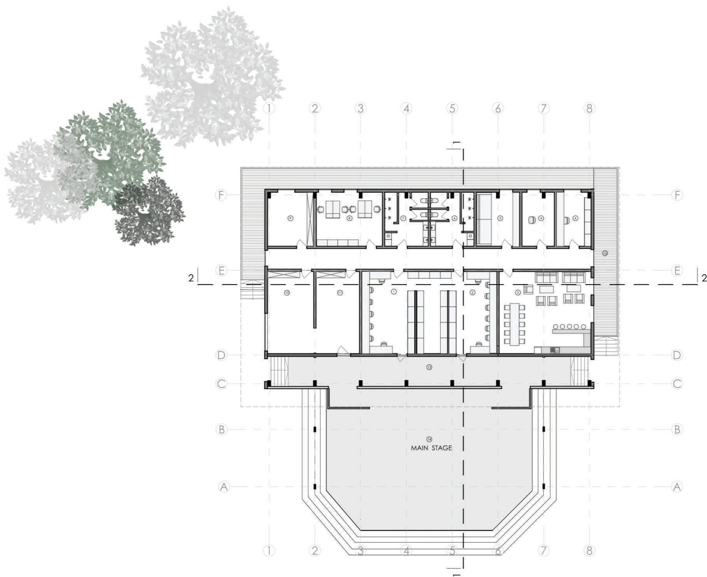
PLAN OF WORK AREA SCALE: 1:200
