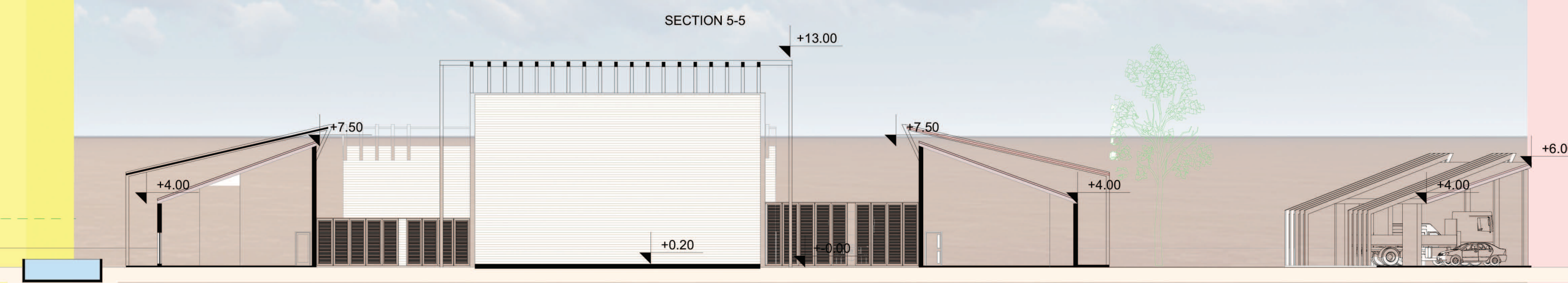
SECTION 6-6
