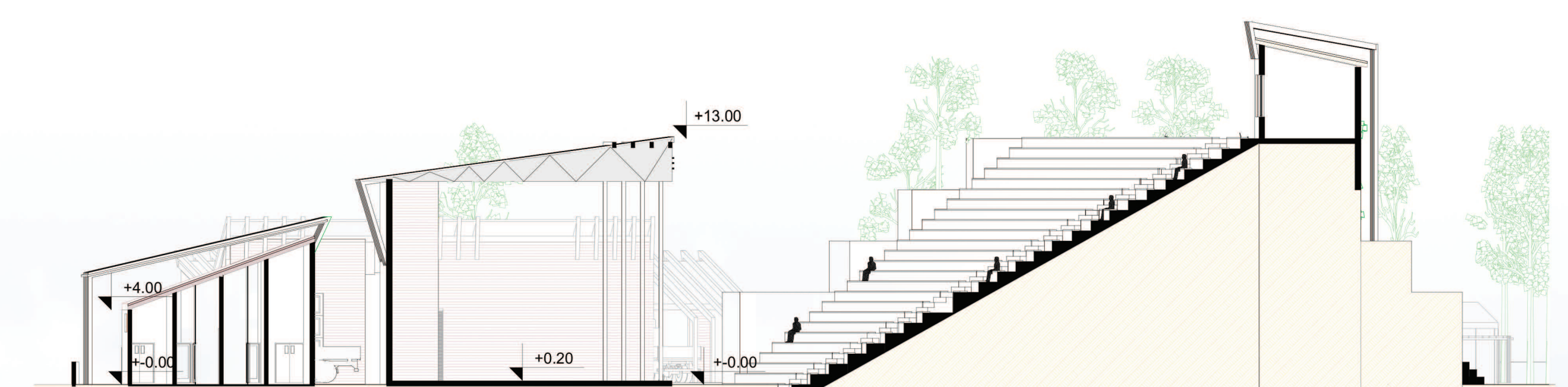
SECTION 2-2
