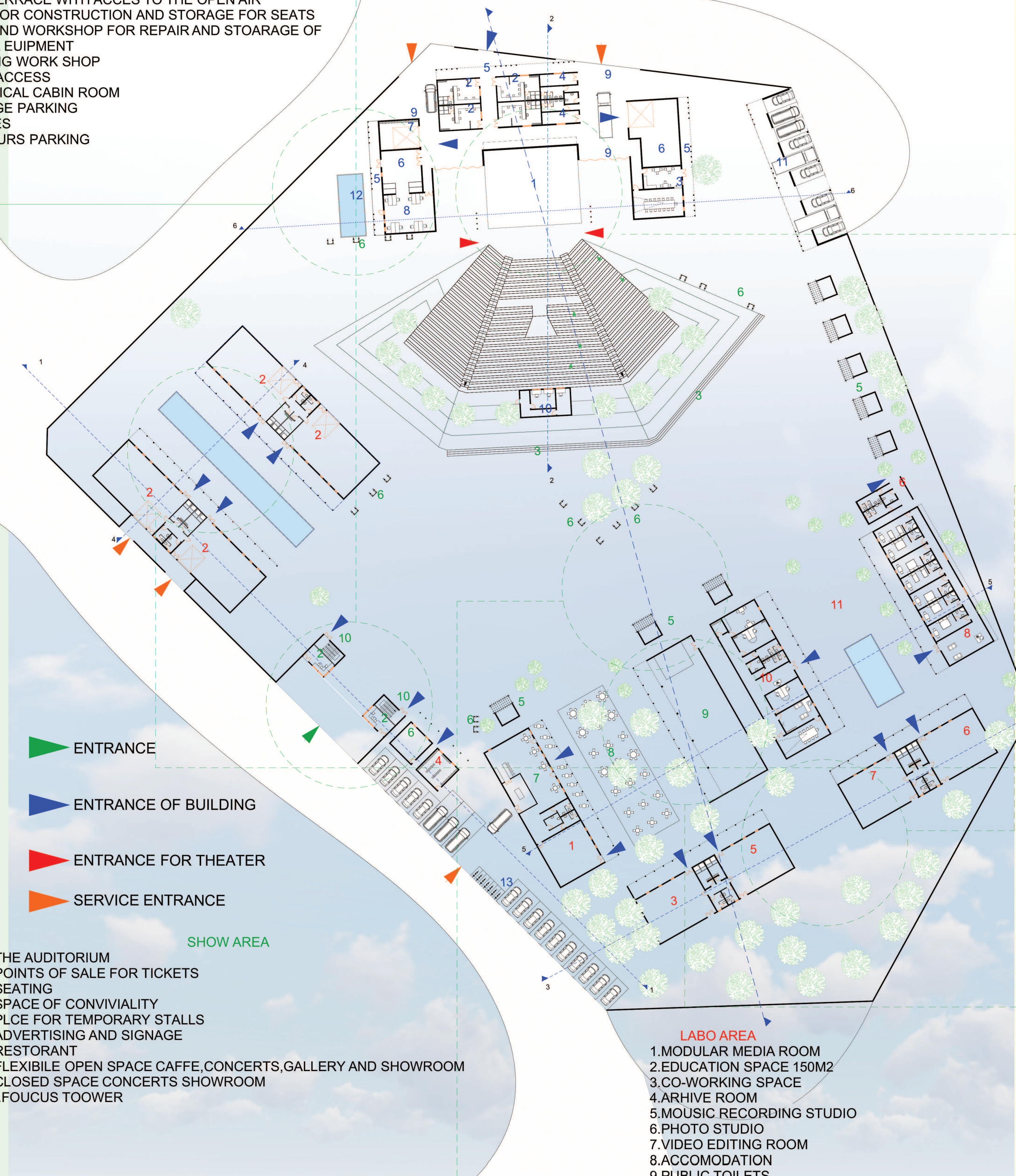
GROUND FLOOR
