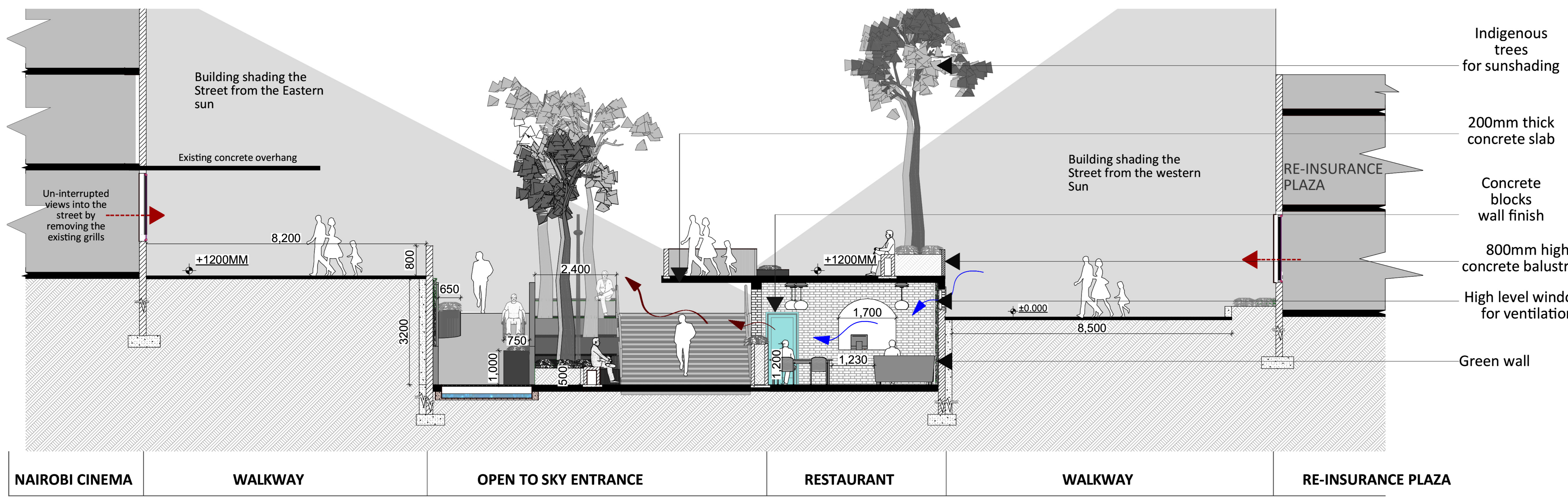
SECTION 02 SCALE 1:50
