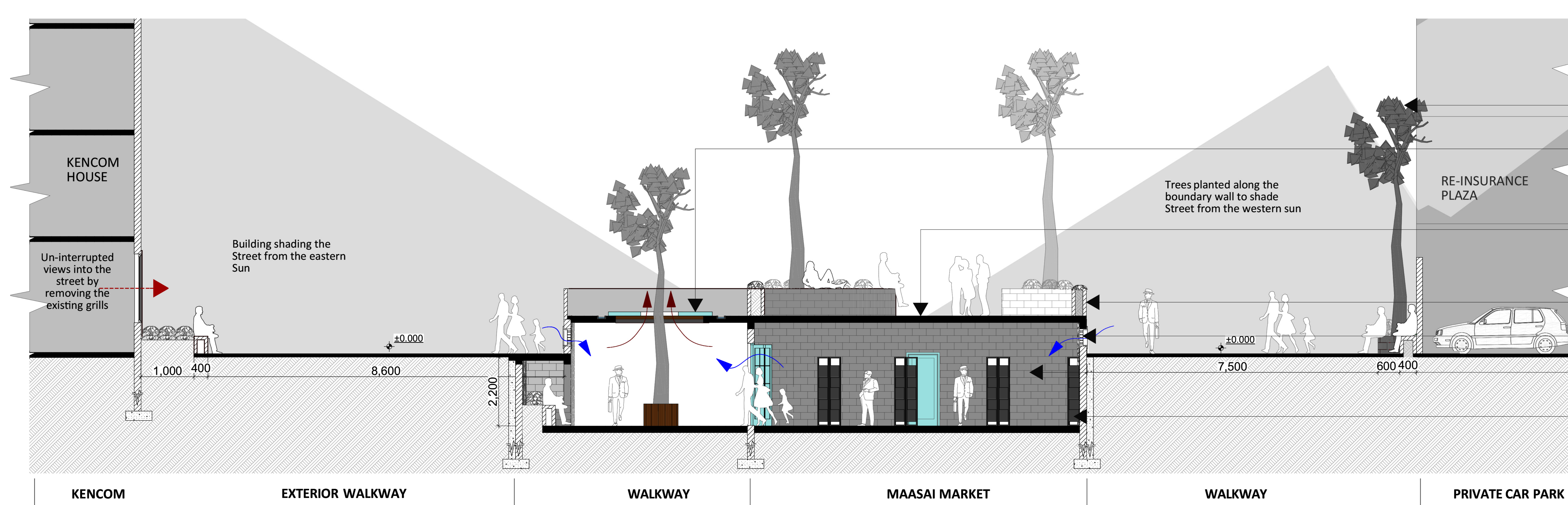
SECTION 03 SCALE 1:50
